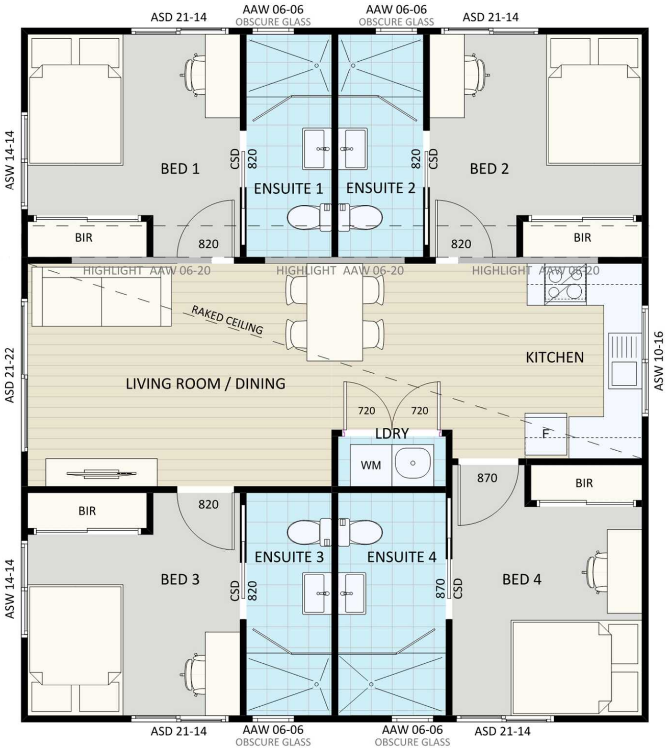
FLOORPLAN_FURNITURE_DESIGN_488
