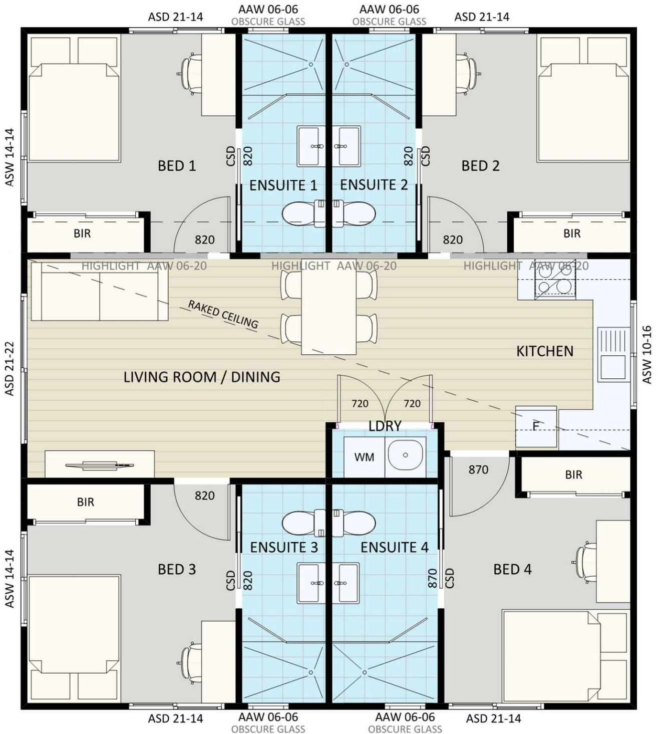
FLOORPLAN_FURNITURE_DESIGN_488
