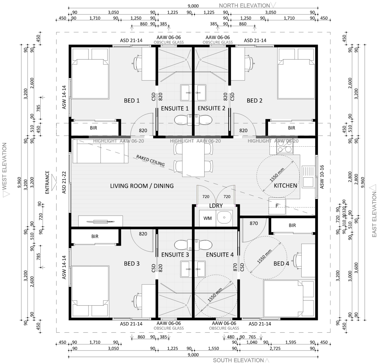
FLOORPLAN_DIMENSION_DESIGN_488
