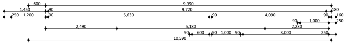
NORTH-EAST ELEVATION
