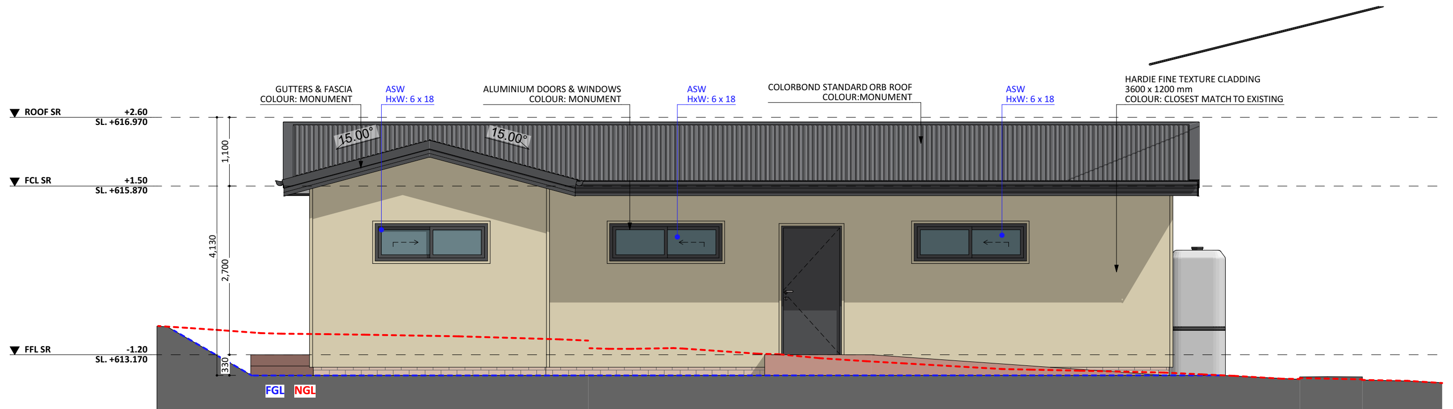
WEST ELEV.
