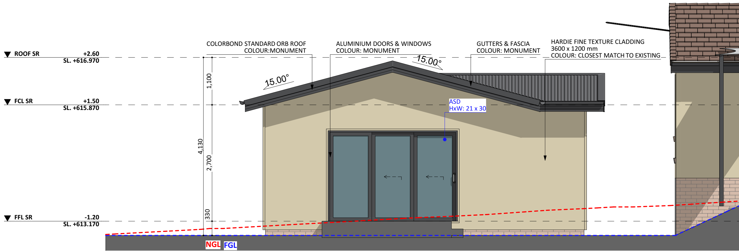
NORTH ELEV.
