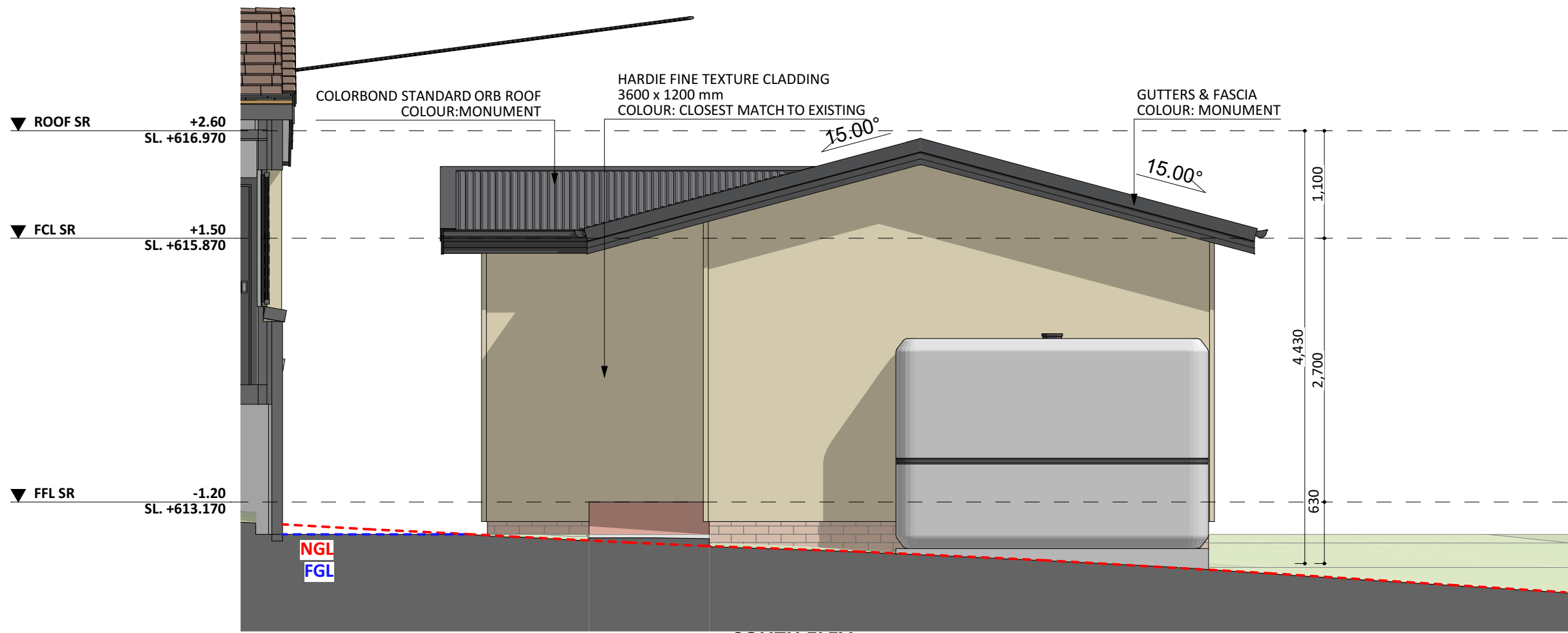
SOUTH ELEV.
