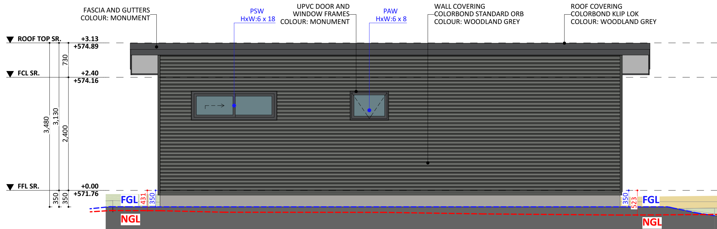
EAST ELEV.
