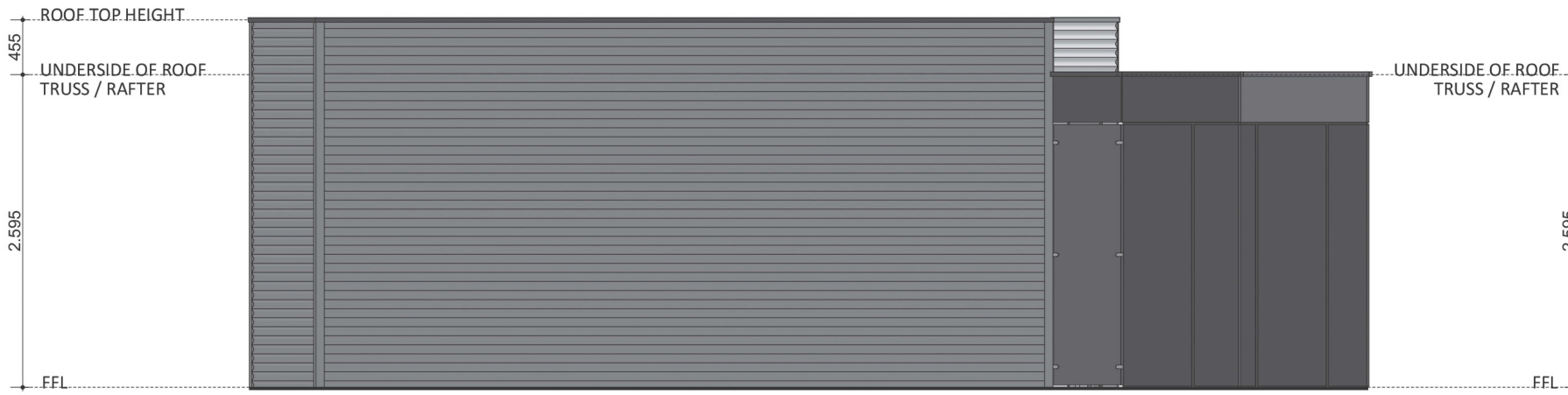
ELEVATION 03
