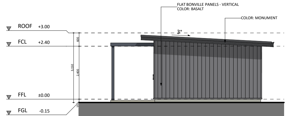
WEST ELEVATION
