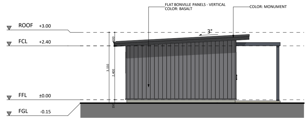
EAST ELEVATION
