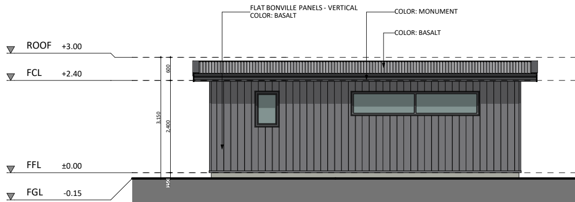
SOUTH ELEVATION
