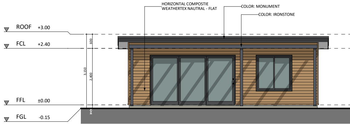
NORTH ELEVATION
