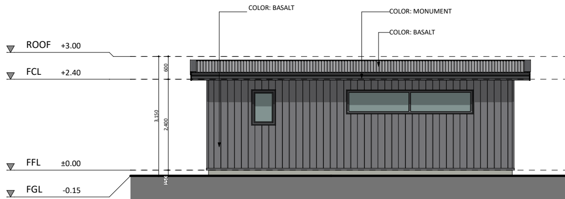
SOUTH ELEVATION
