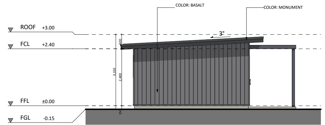
EAST ELEVATION
