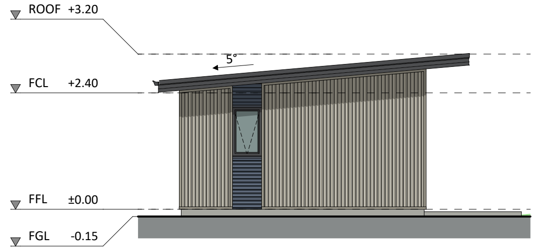
EAST ELEVATION
