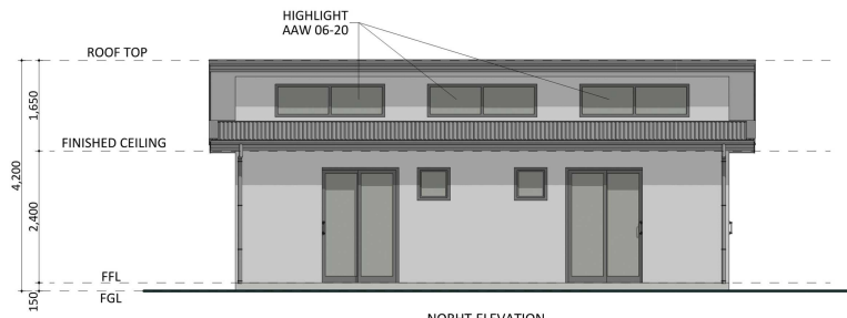
NORHT ELEVATION
