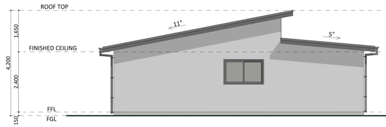
EAST ELEVATION
