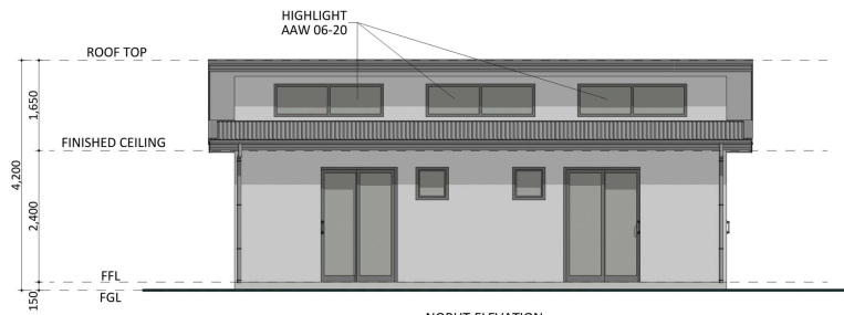
NORHT ELEVATION
