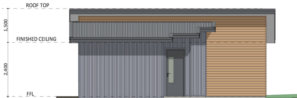
SOUTH ELEVATION
