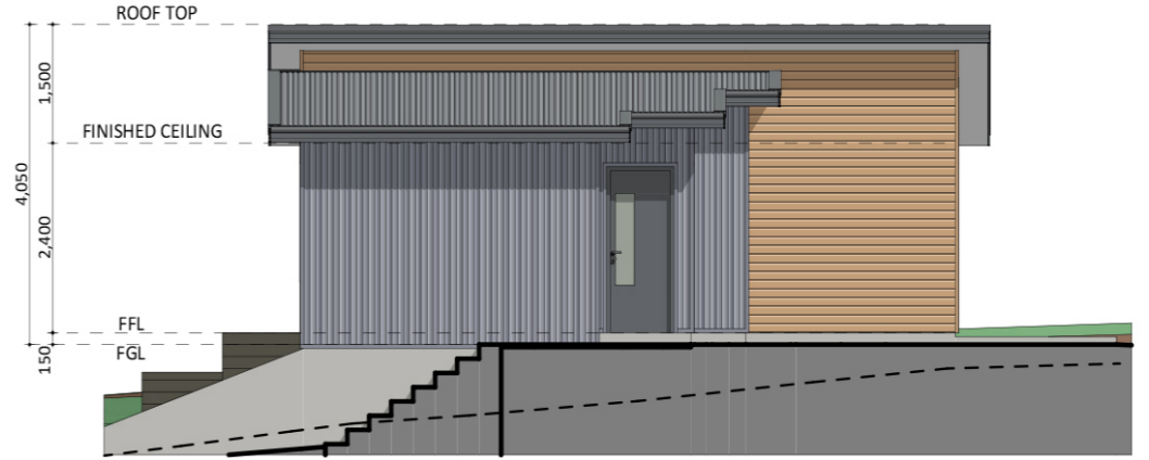
SOUTH ELEVATION
