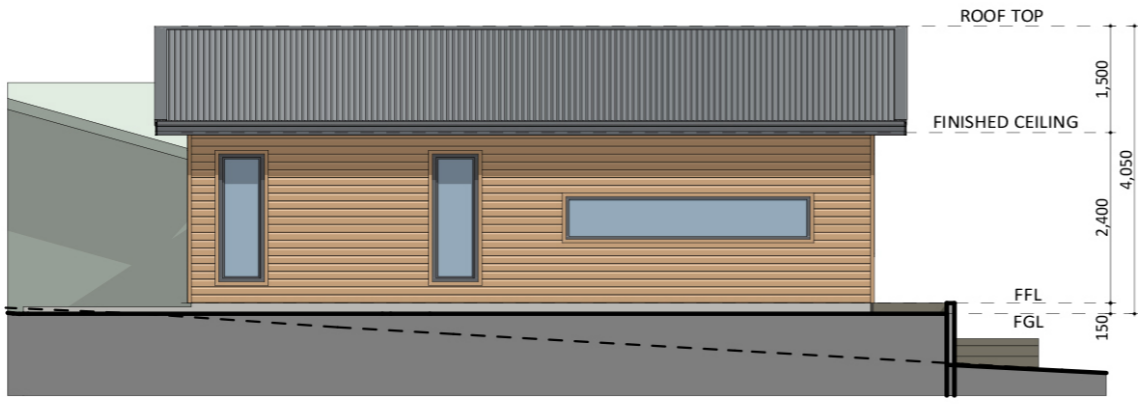
NORTH ELEVATION
