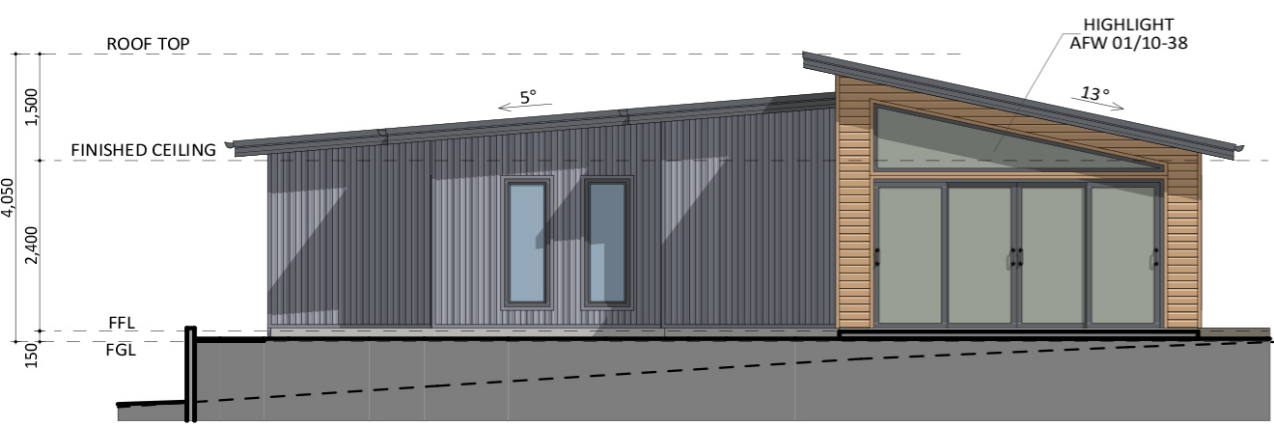
EAST ELEVATION
