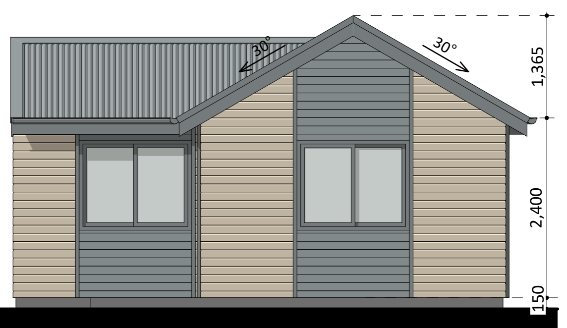
WEST ELEVATION
