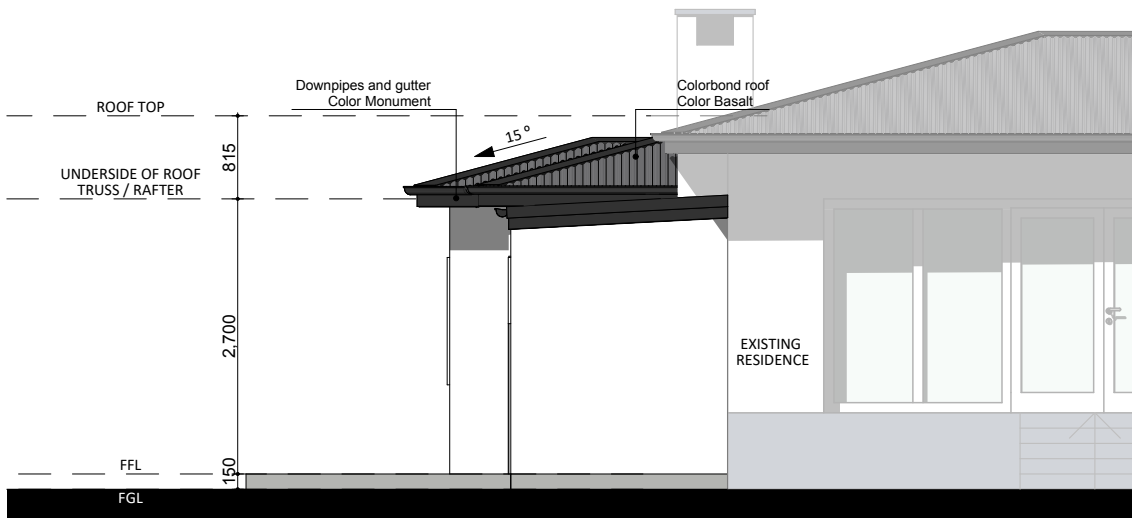
WEST ELEVATION
