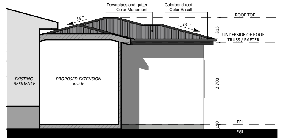
SOUTH ELEVATION
