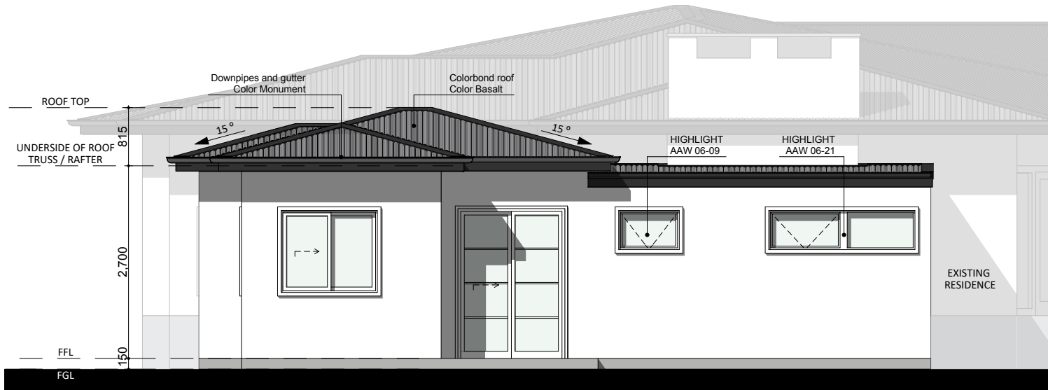
NORTH ELEVATION
