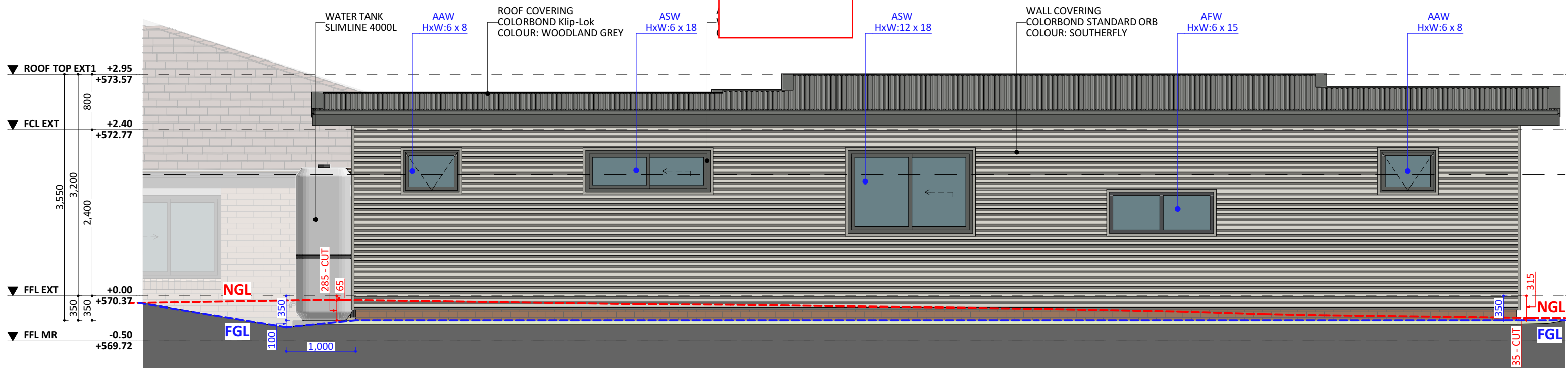
EAST ELEV.
