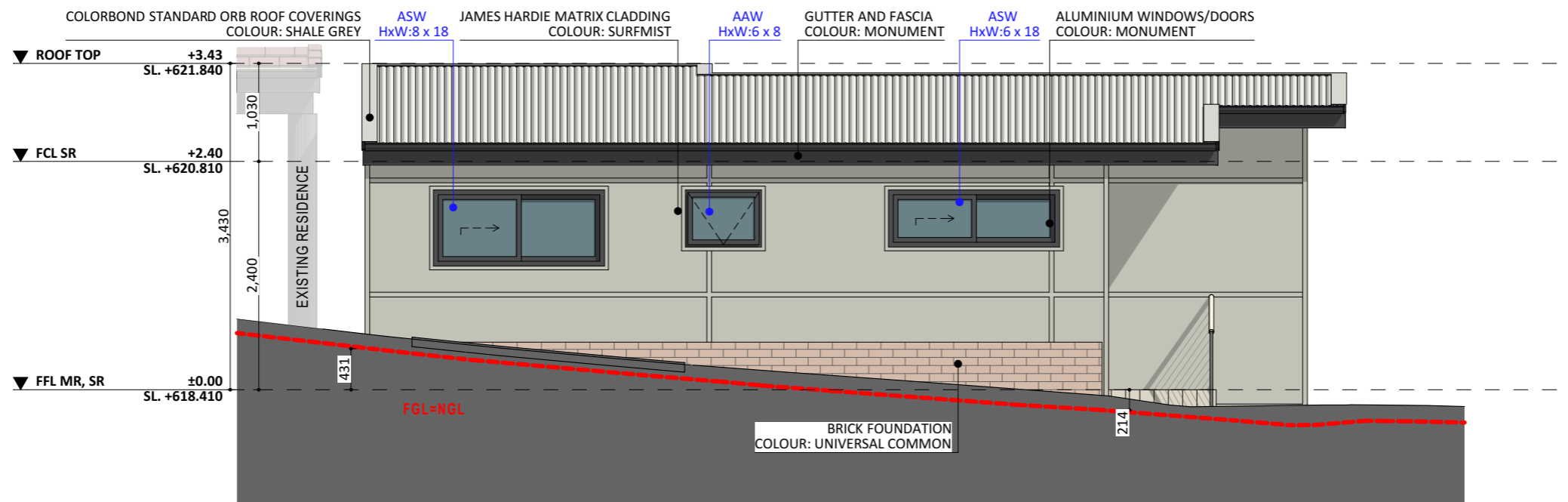
WEST ELEV.
