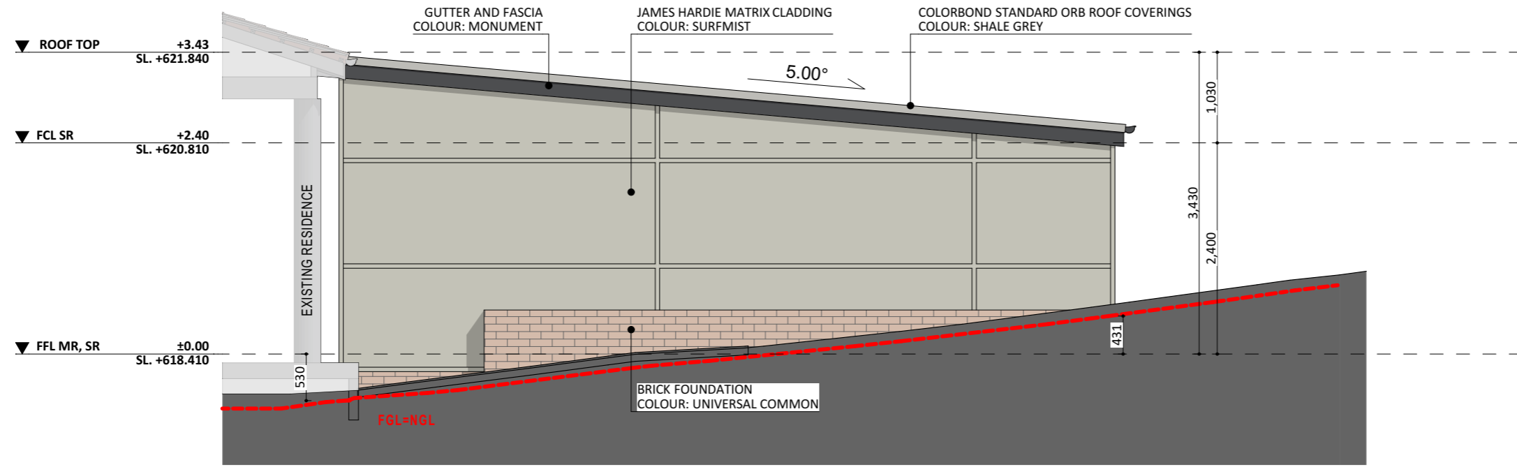
NORTH ELEV.
