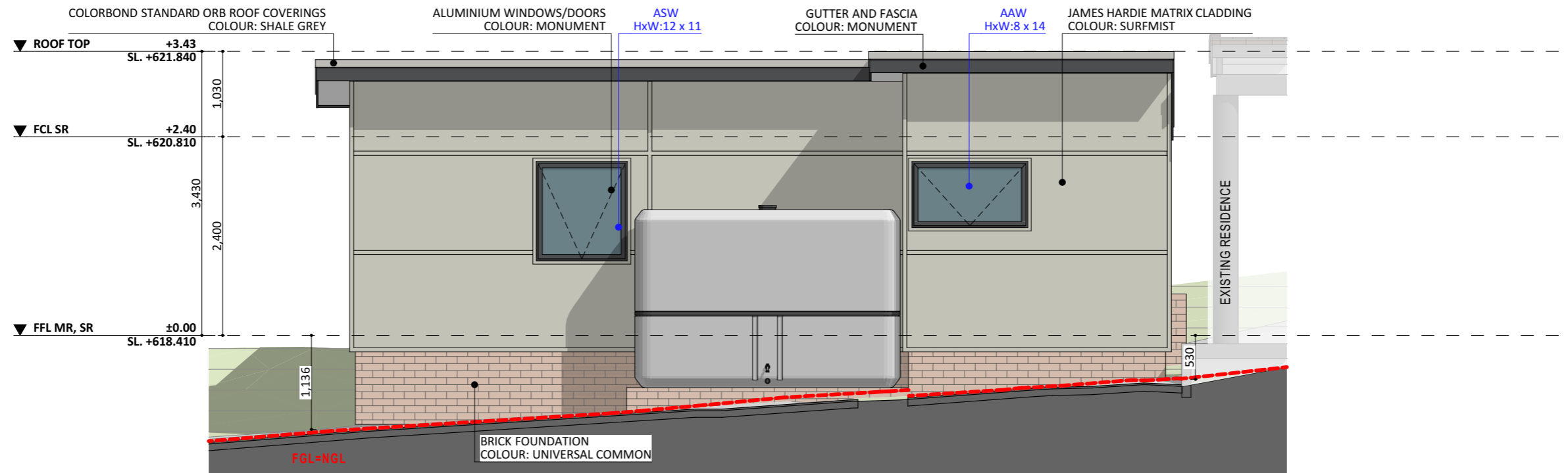
EAST ELEV.
