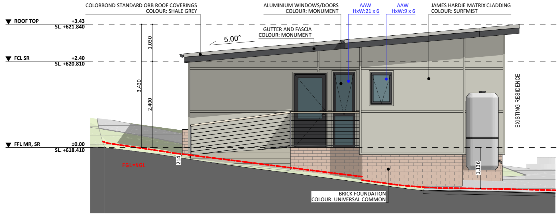
SOUTH ELEV.
