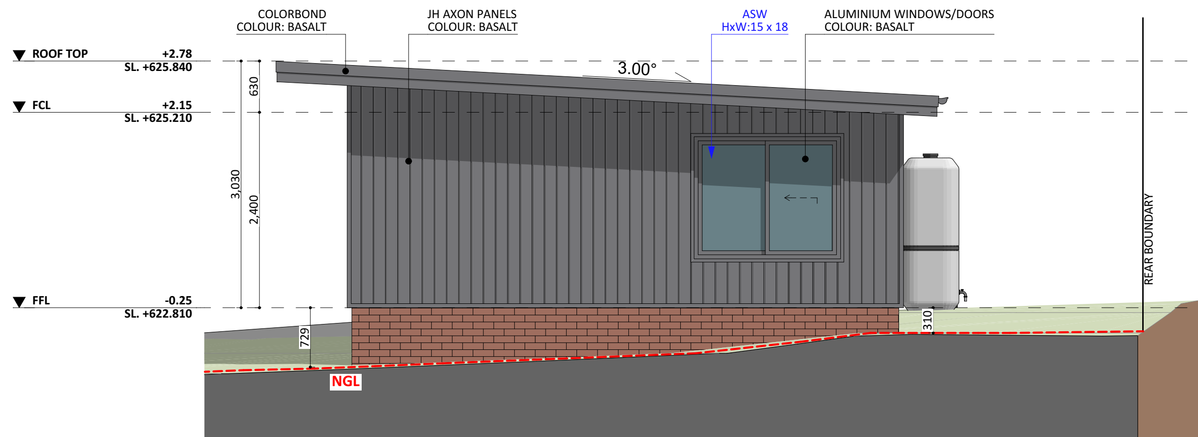
WEST ELEV.
