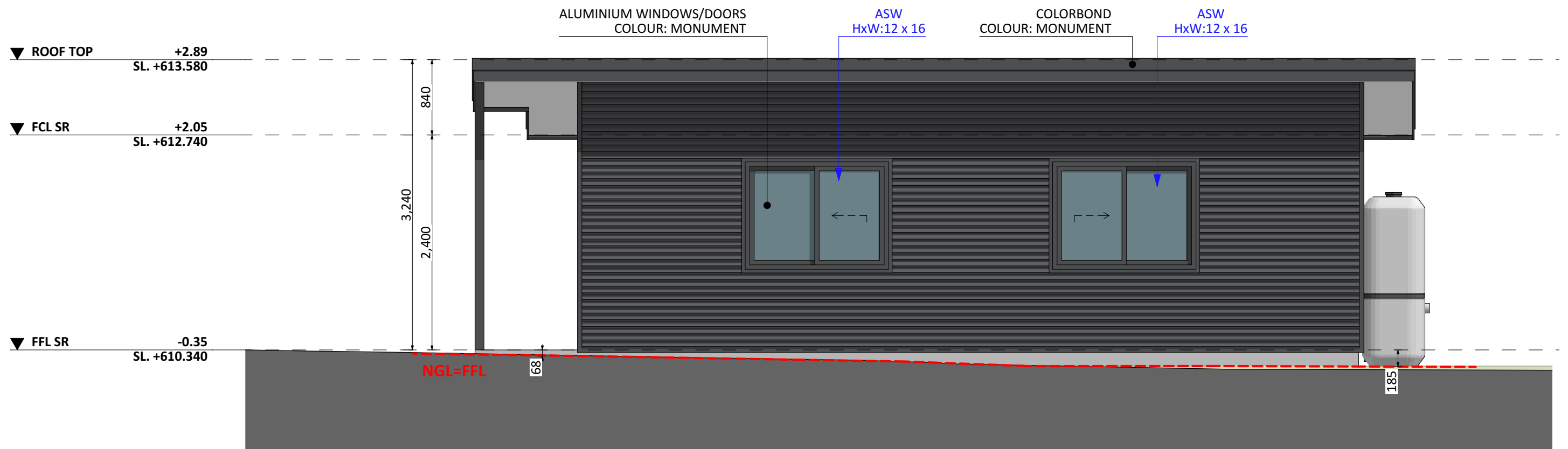
NORTH ELEV.
