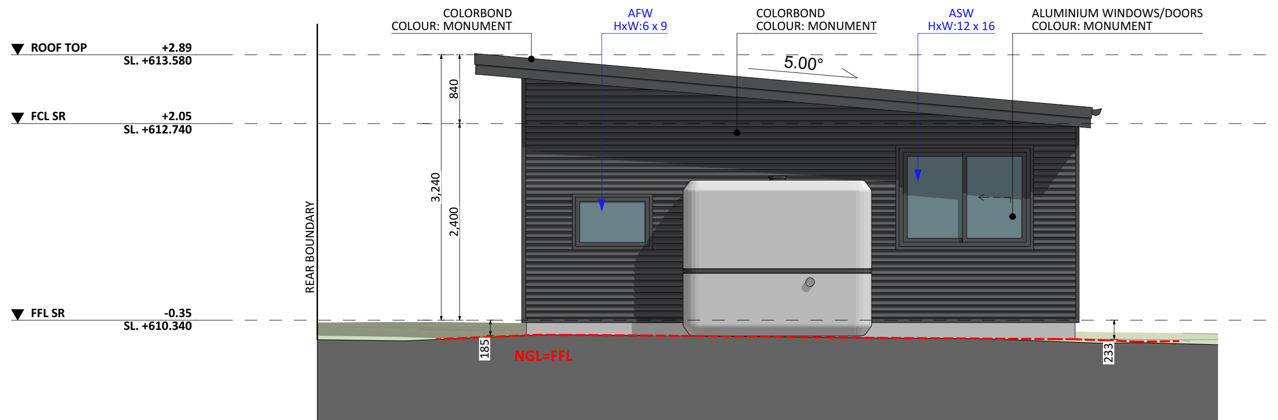
WEST ELEV.
