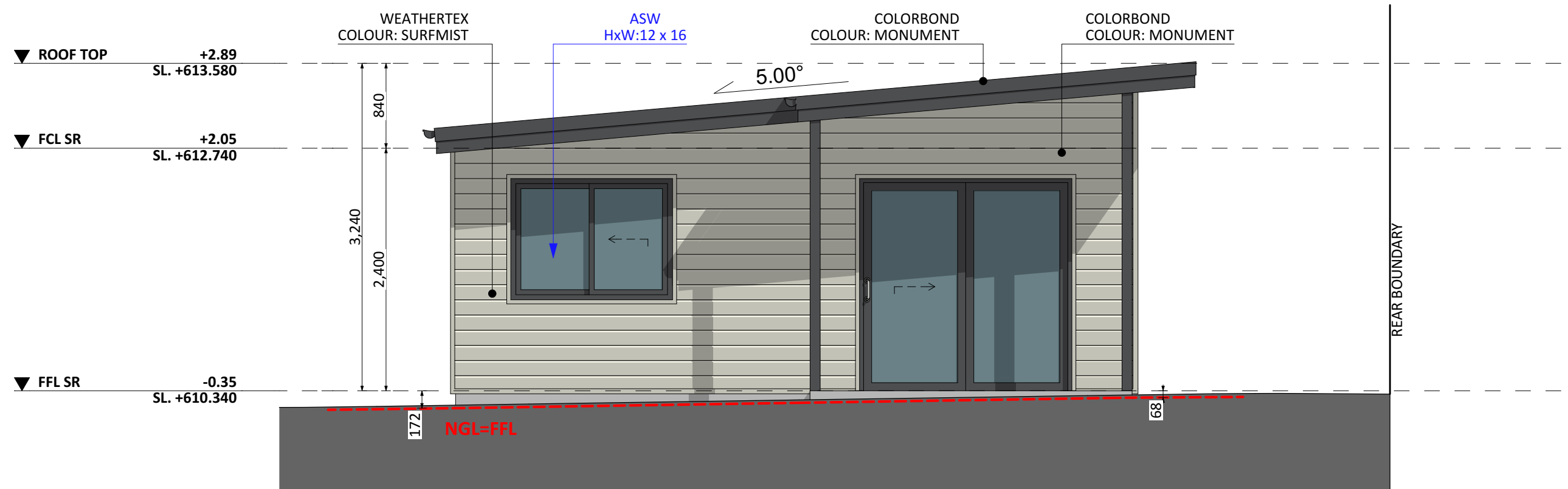
EAST ELEV.
