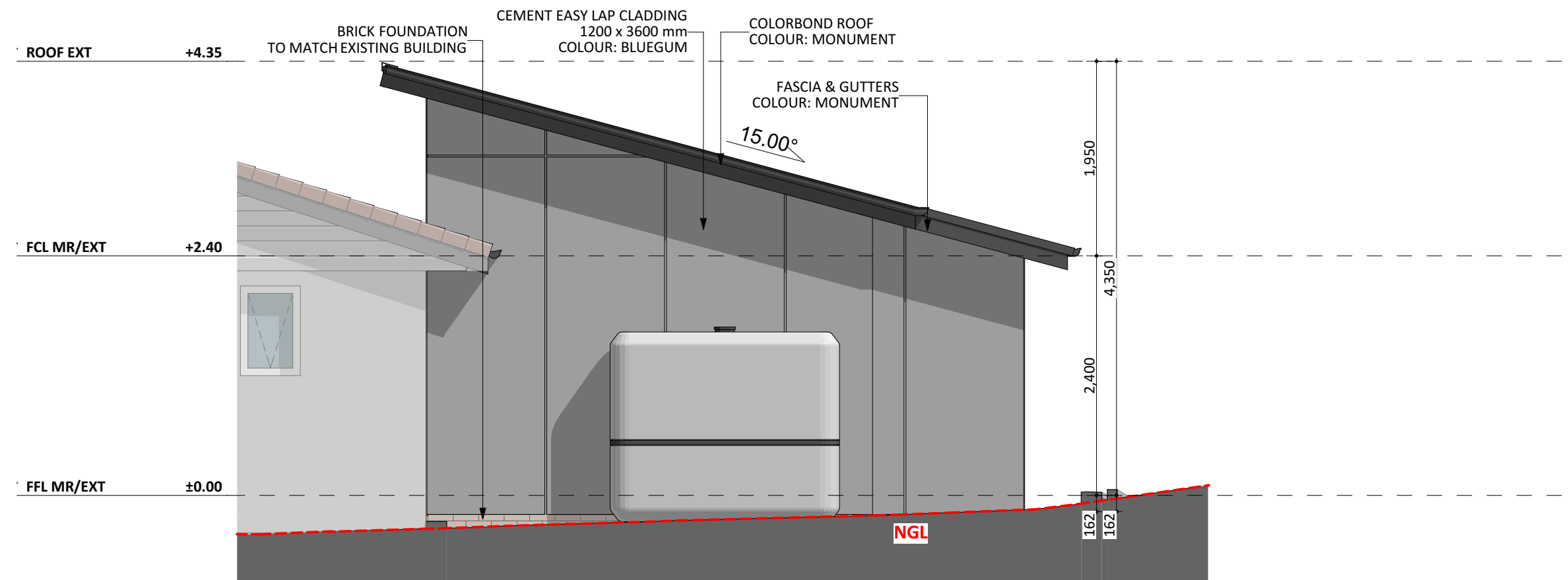
WEST ELEV.
