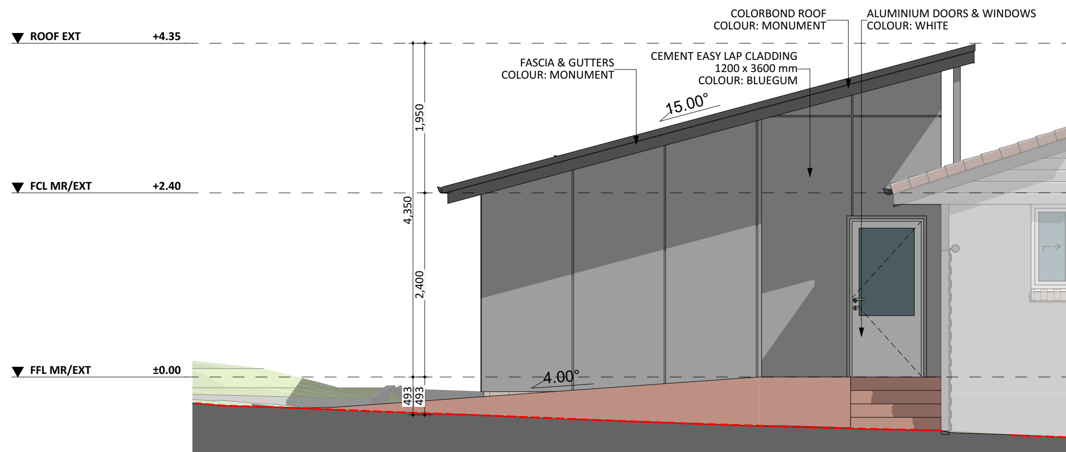
EAST ELEV.
