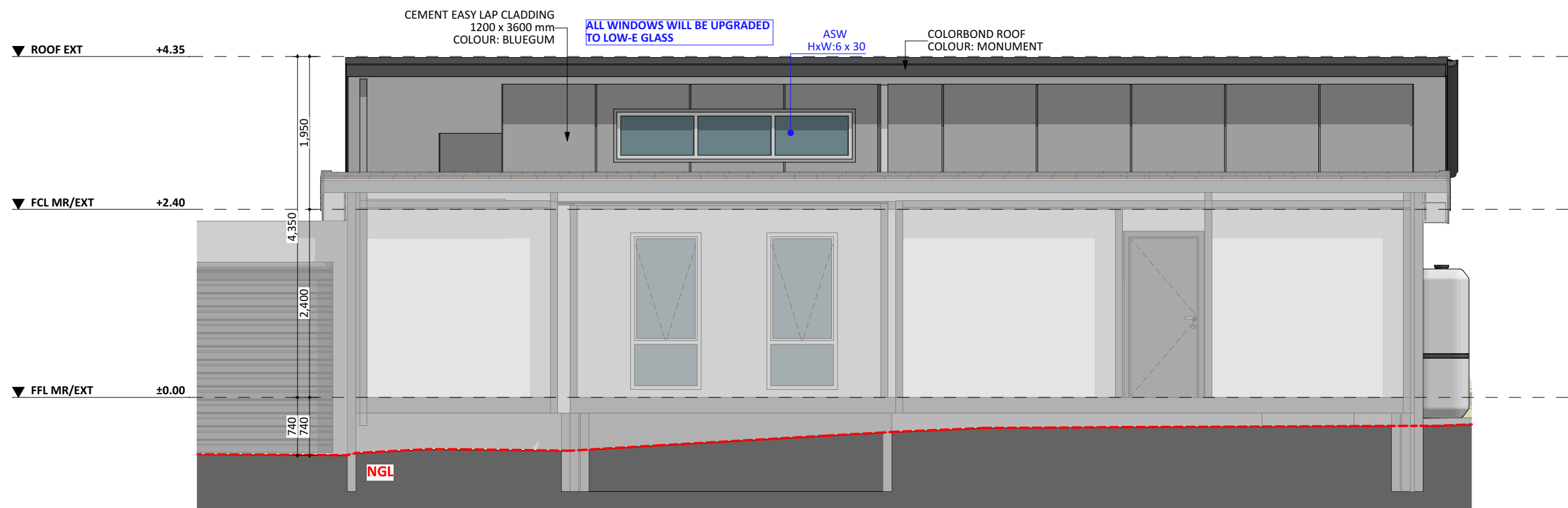
NORTH ELEV.
