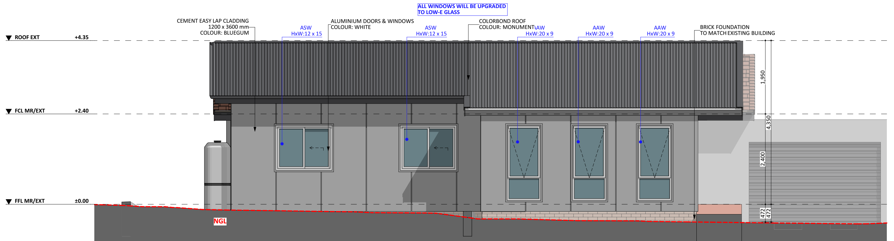
SOUTH ELEV.
