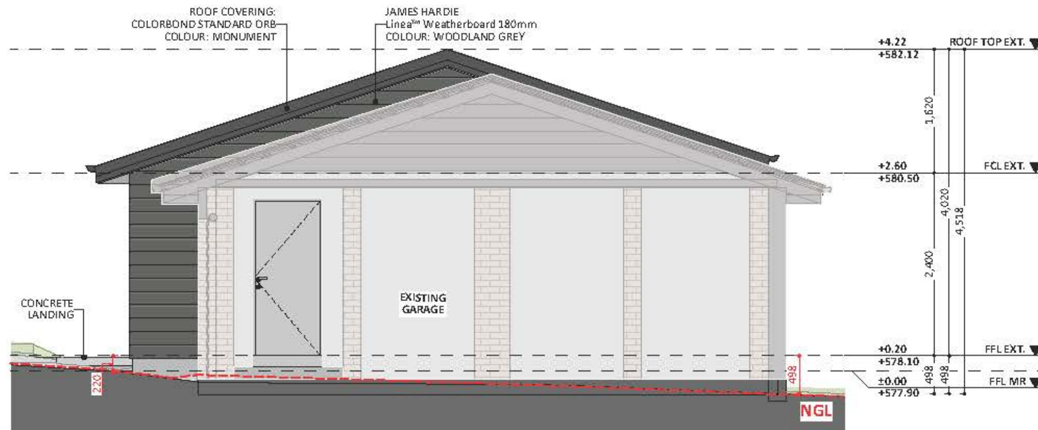
EAST ELEV.
