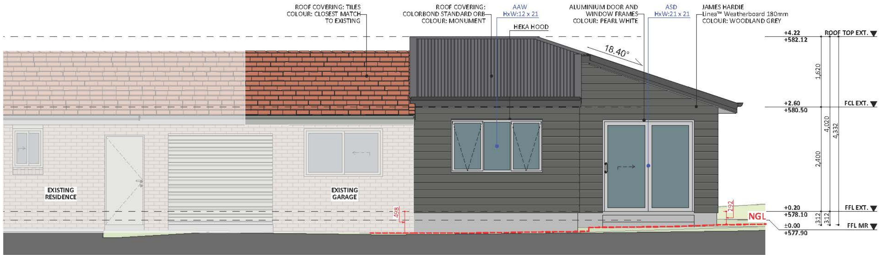
NORTH ELEV.
