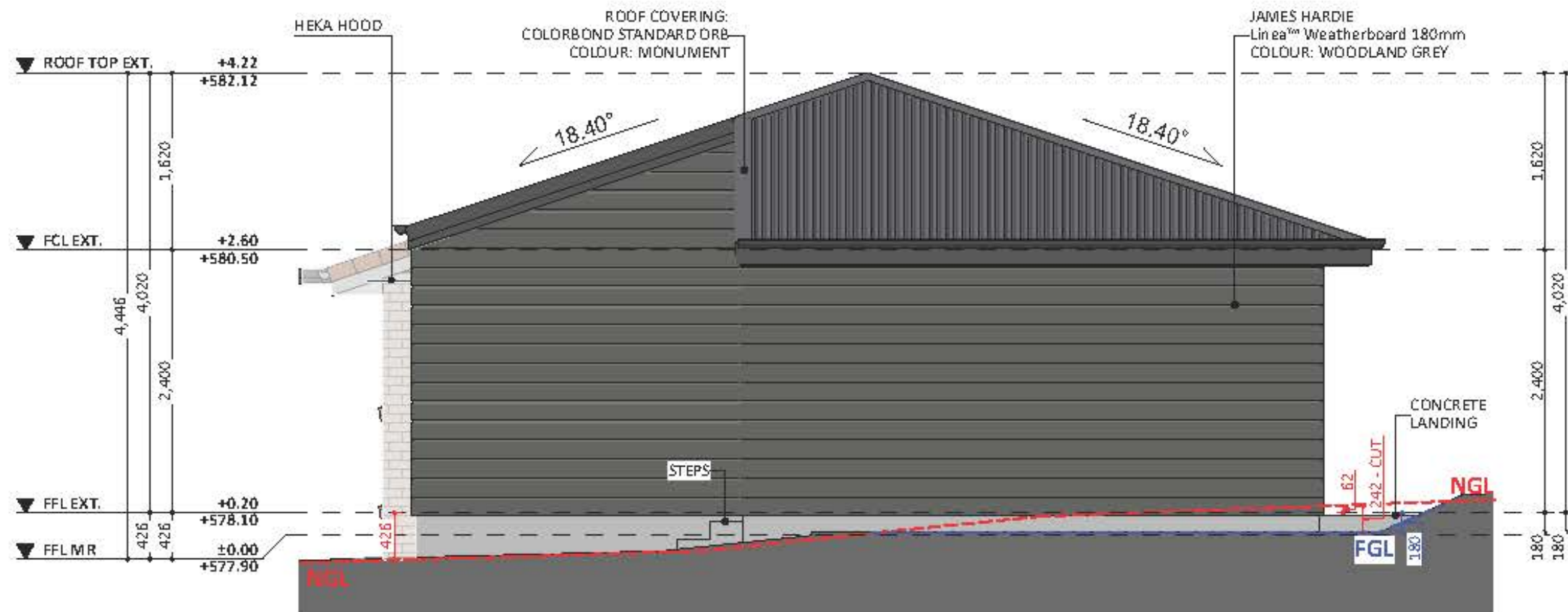
WEST ELEV.
