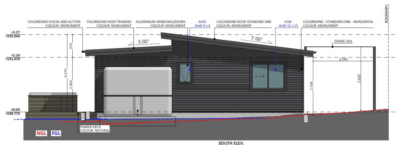
SOUTH ELEV.
