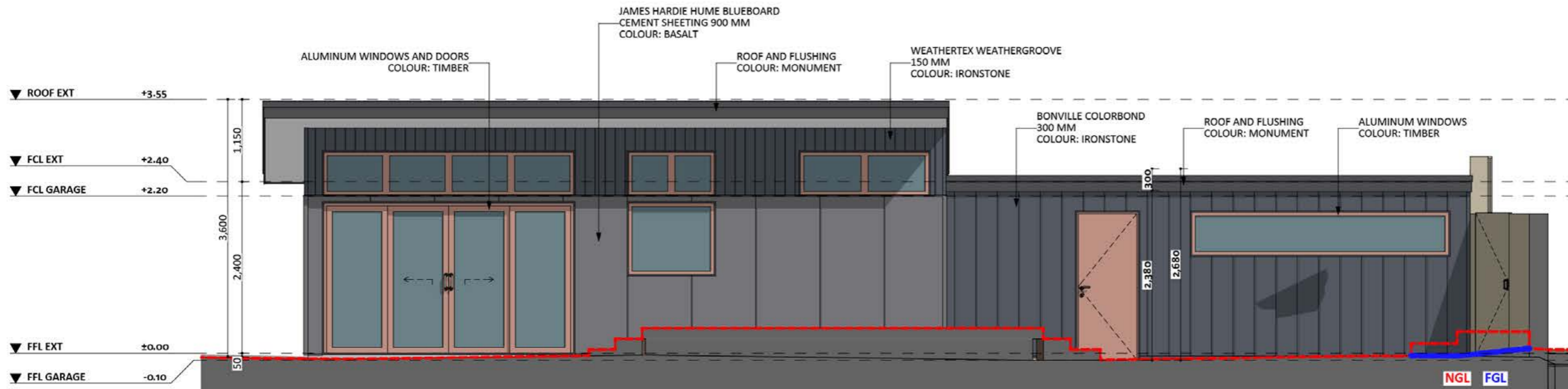
NORTH-EAST ELEVATION
