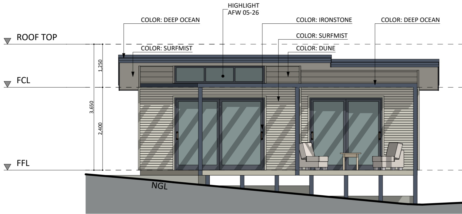
NORTH-WEST ELEVATION
