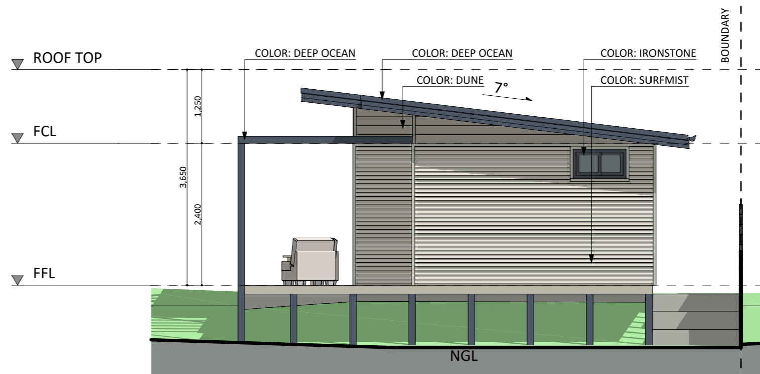
SOUTH-WEST ELEVATION
