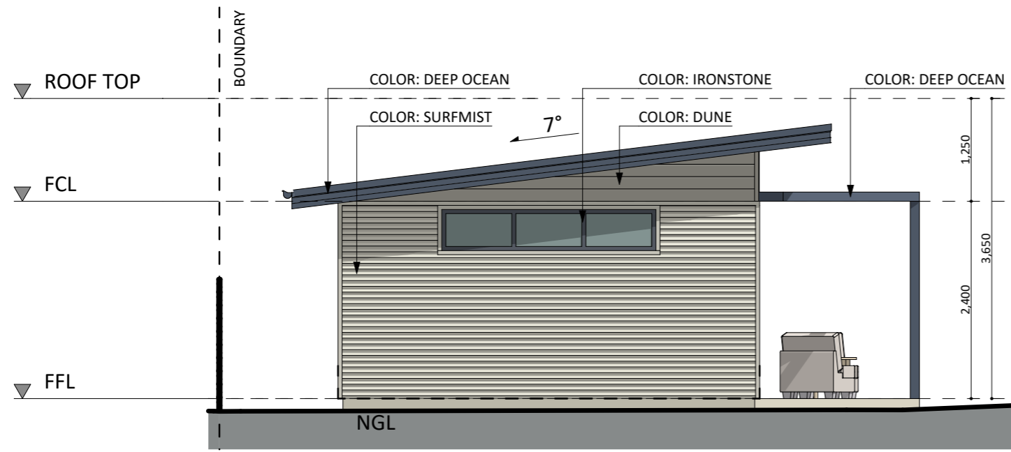
NORTH-EAST ELEVATION
