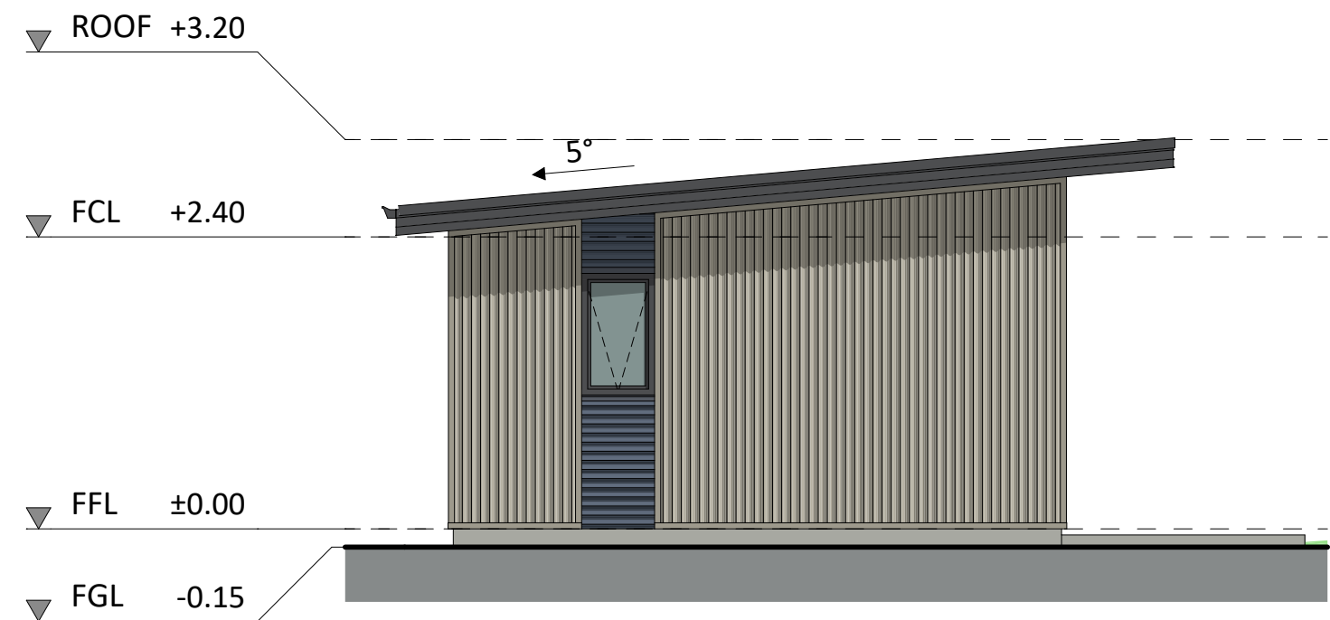
EAST ELEVATION
