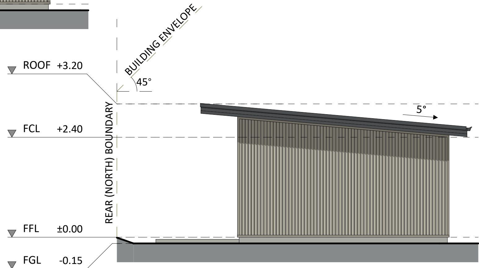
WEST ELEVATION
