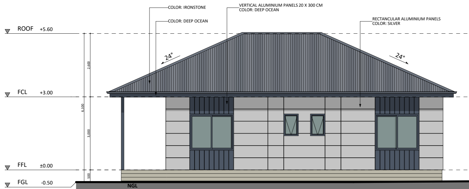
SOUTH ELEVATION
