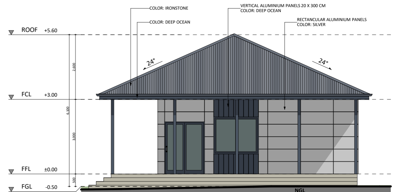
WEST ELEVATION
