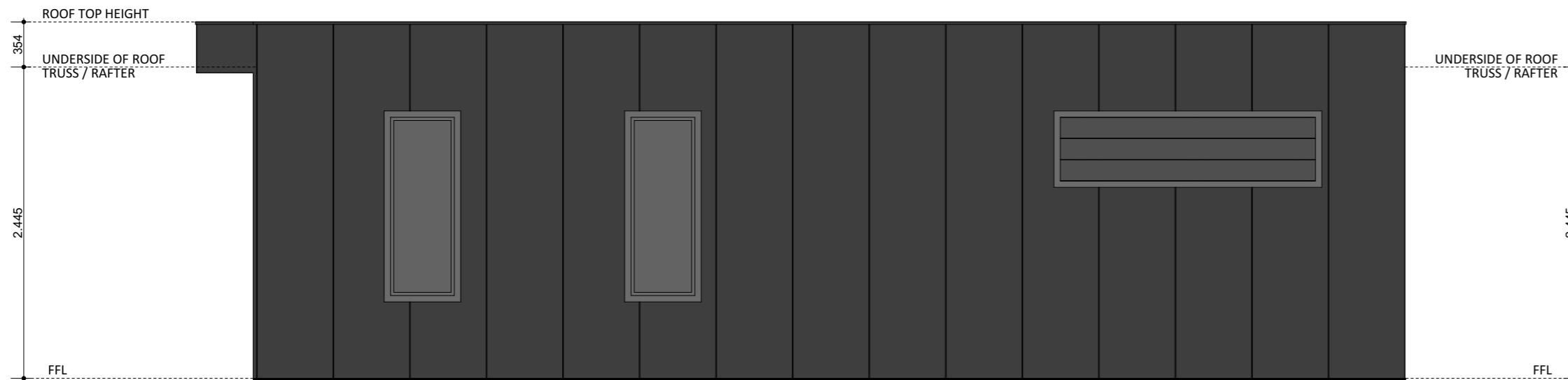
ELEVATION 03
