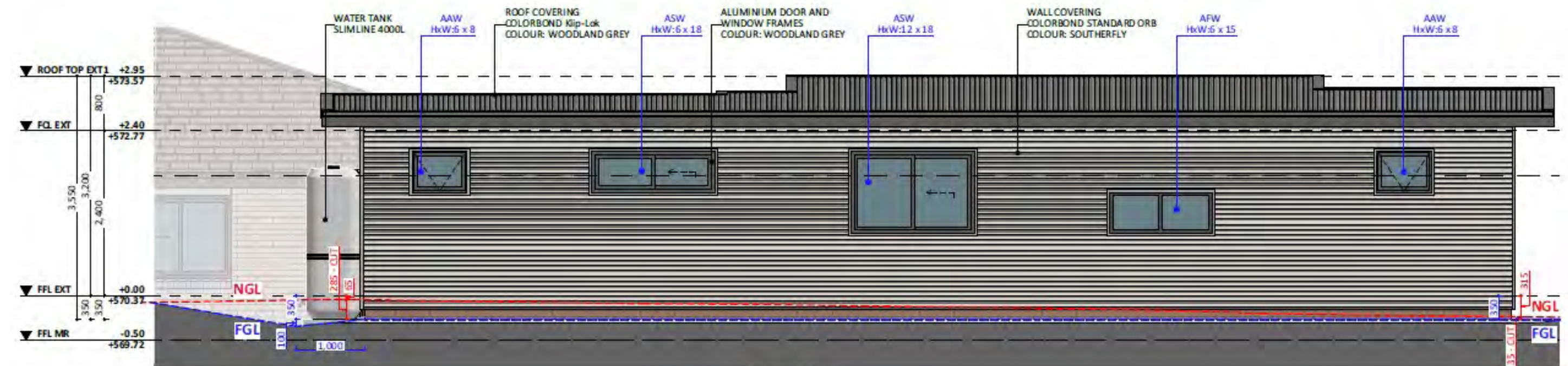
EAST ELEV.
