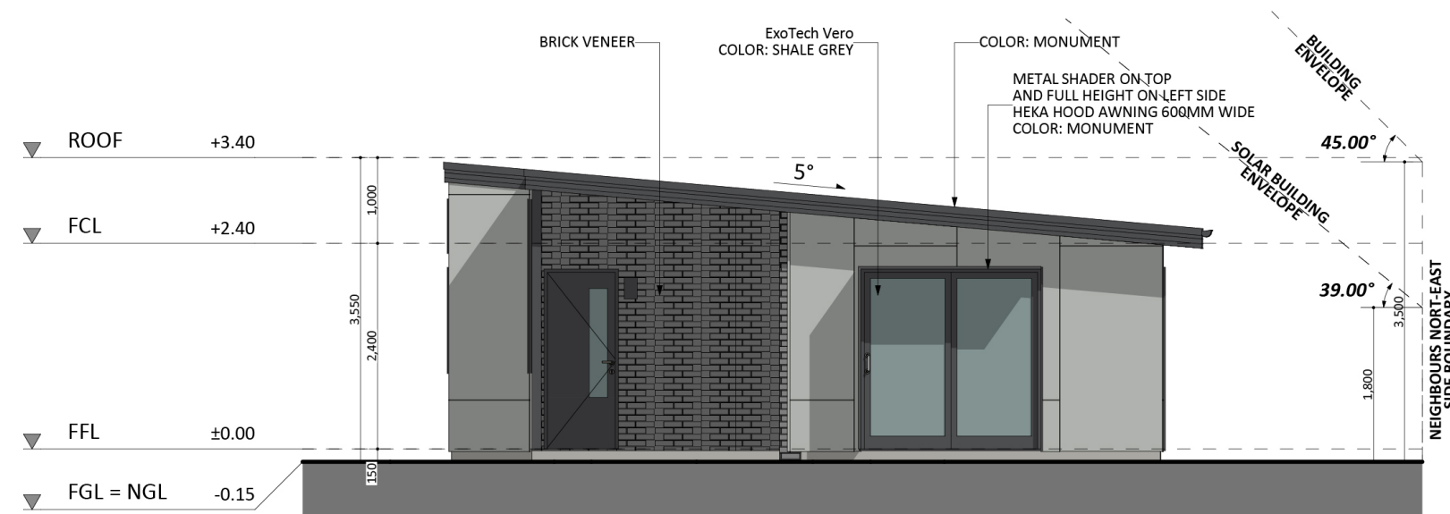
NORTH-WEST ELEVATION
