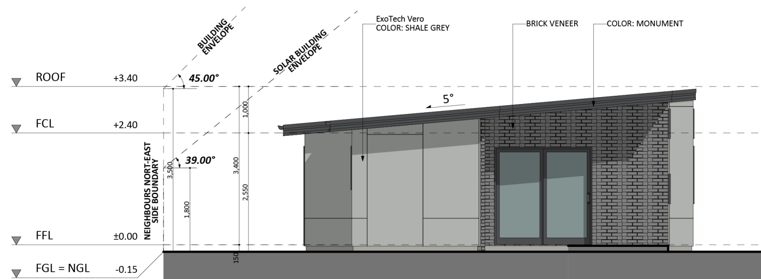
SOUTH-EAST ELEVATION
