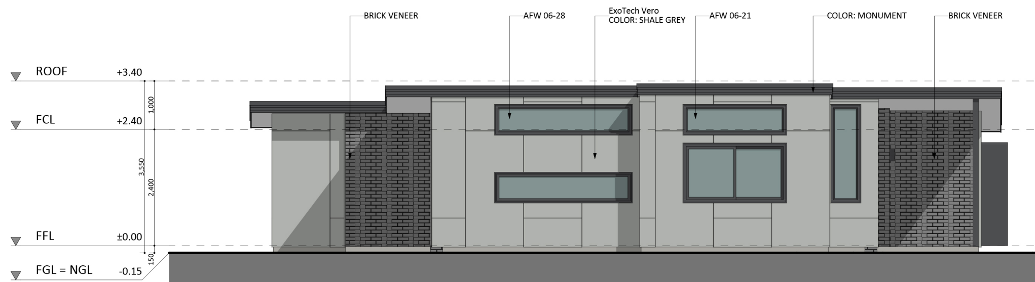
NORTH-EAST ELEVATION
