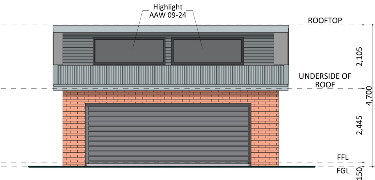
NORTH ELEVATION
