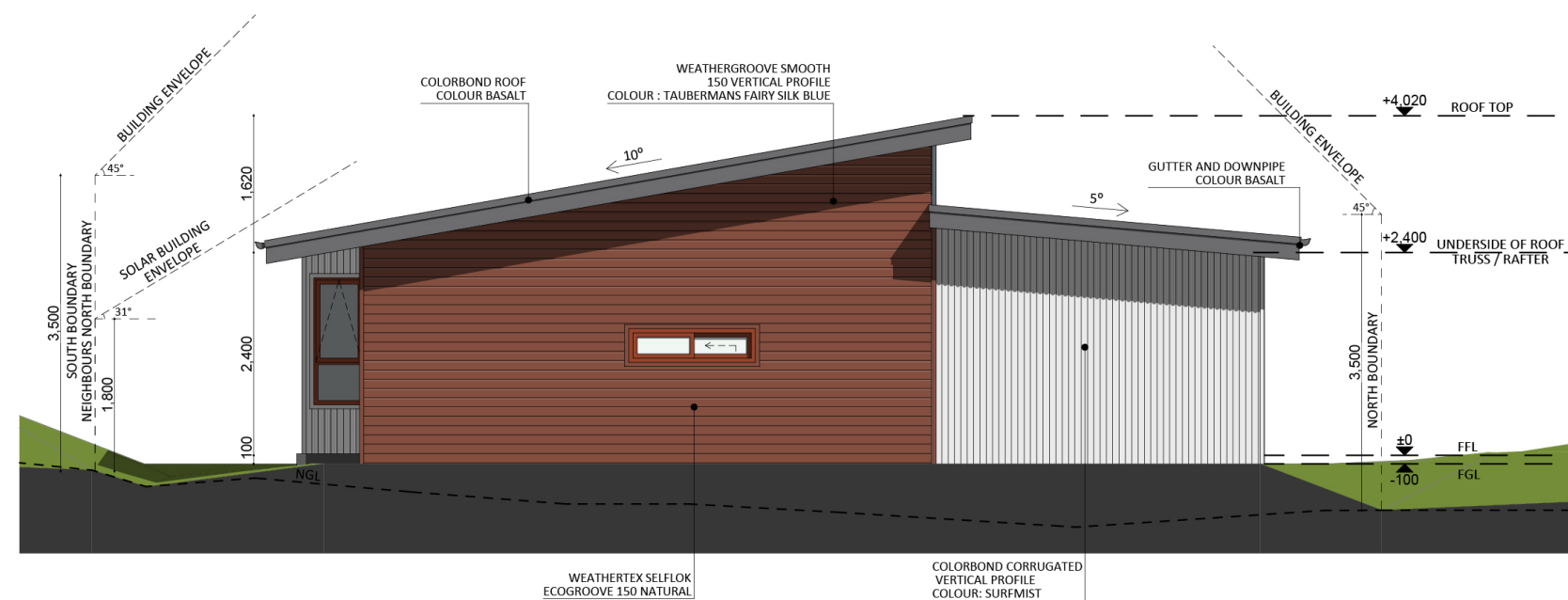
EAST ELEVATION
