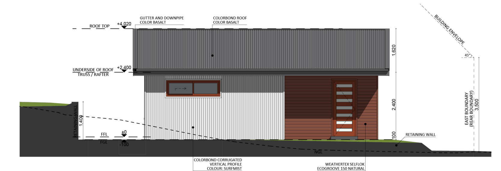
SOUTH ELEVATION
