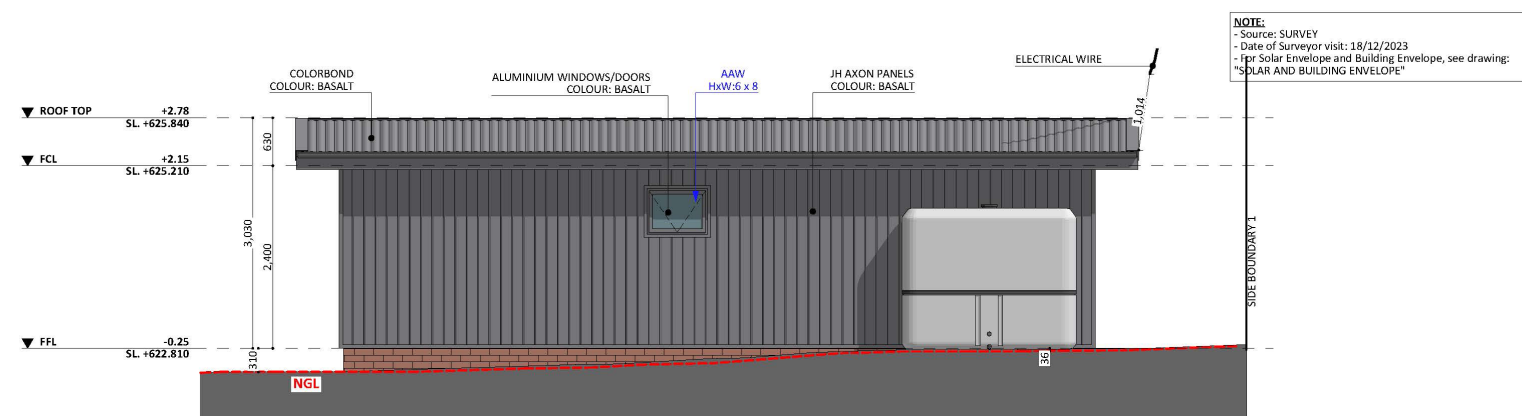
SOUTH ELEV.
