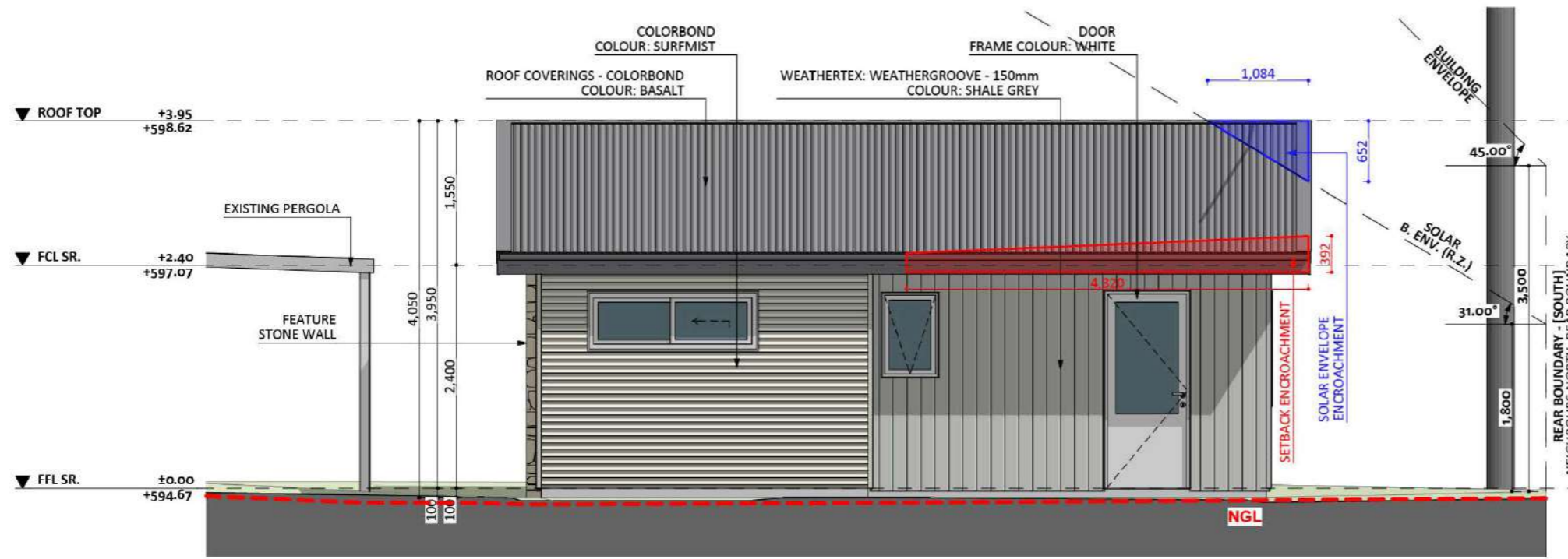
ELEVATION 03
