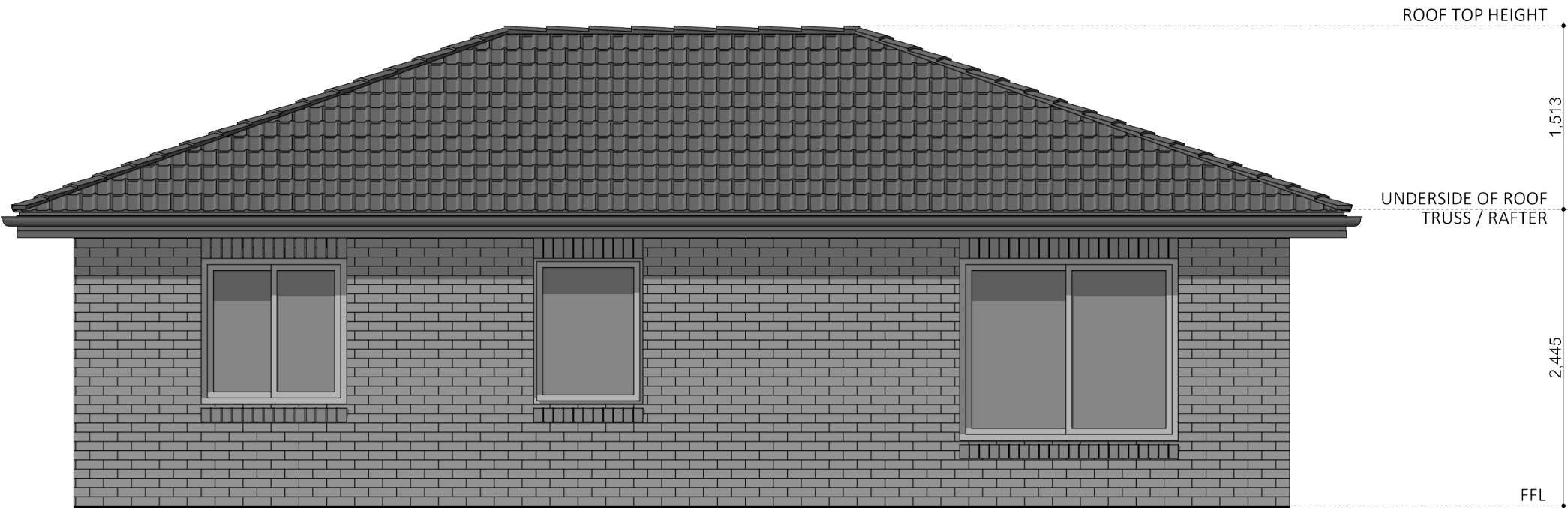
ELEVATION 03
