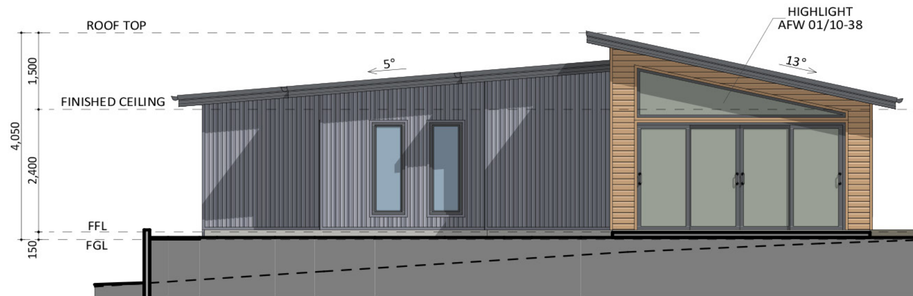
EAST ELEVATION
