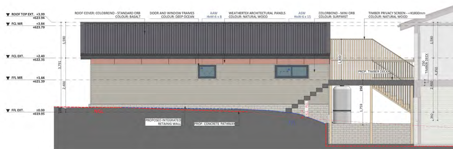
SOUTH-WEST ELEV. - EXT.
