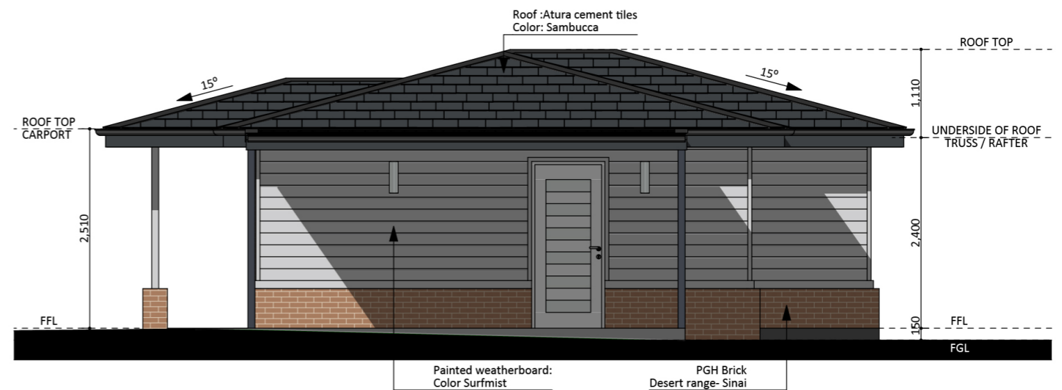
WEST ELEVATION
