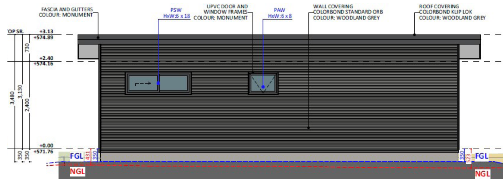
EAST ELEV.
