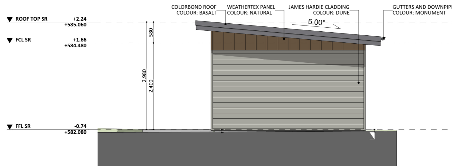
NORTH-EAST ELEV.
