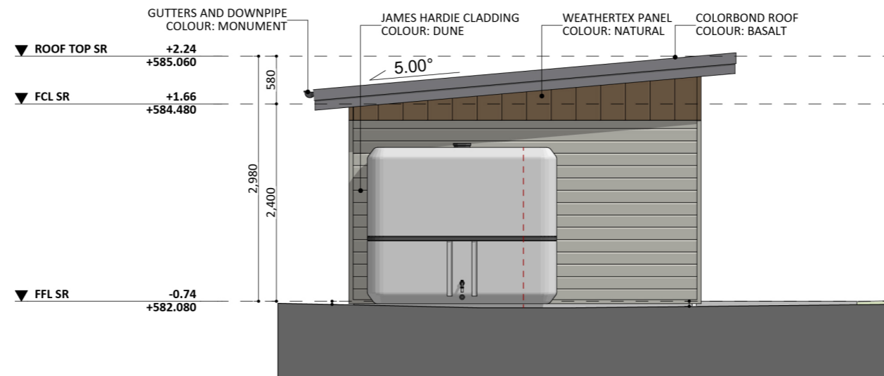
SOUTH-WEST ELEV.
