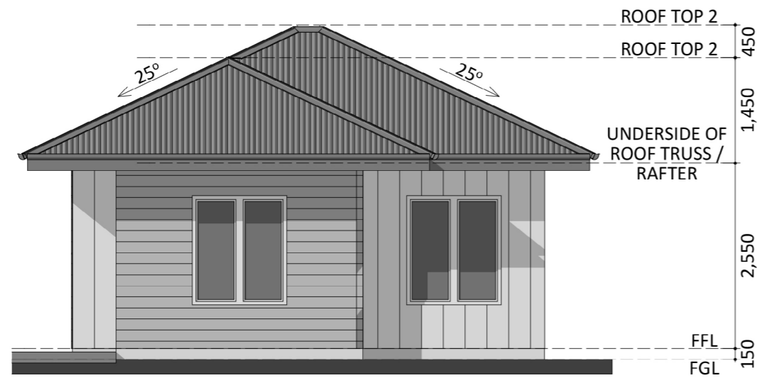
NORTH-WEST ELEVATION
