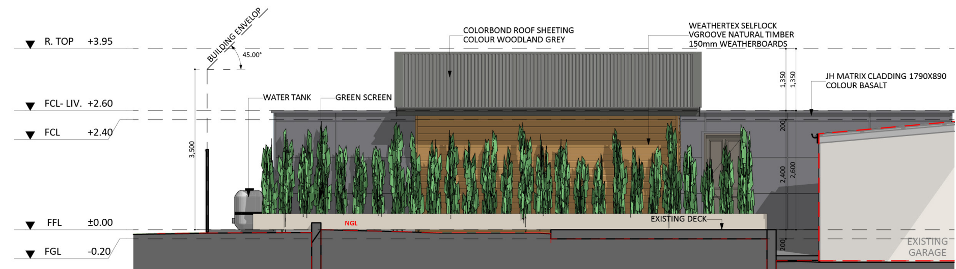
SOUTH ELEVATION
