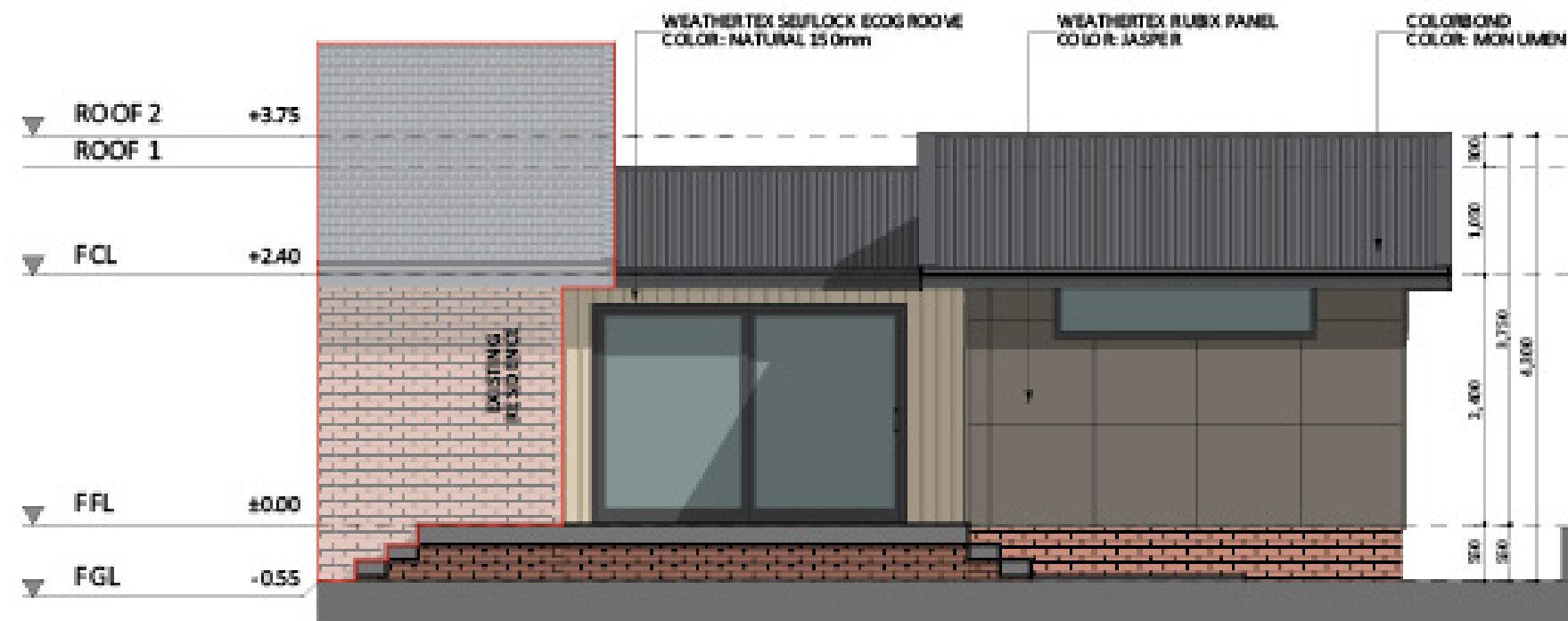
NORTH-WEST ELEVATION - OPT 1
