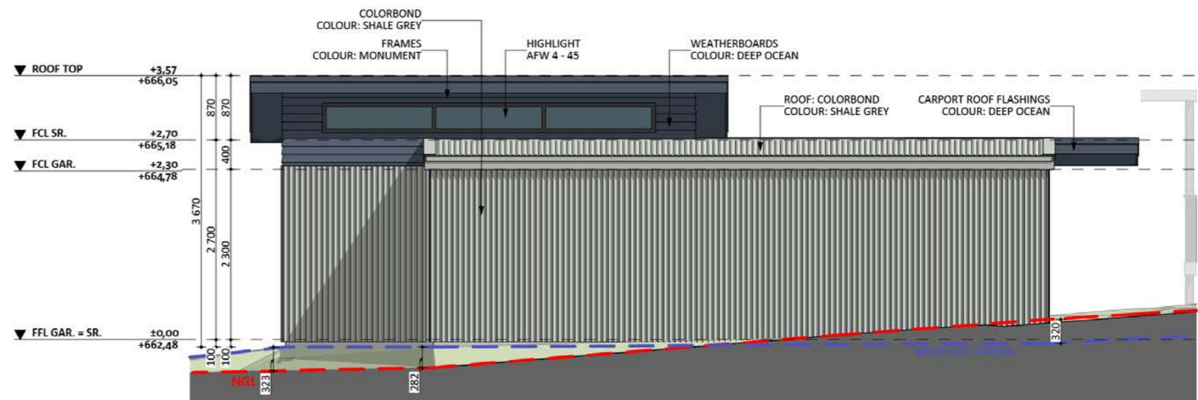
NORTH-WEST ELEVATIONS
