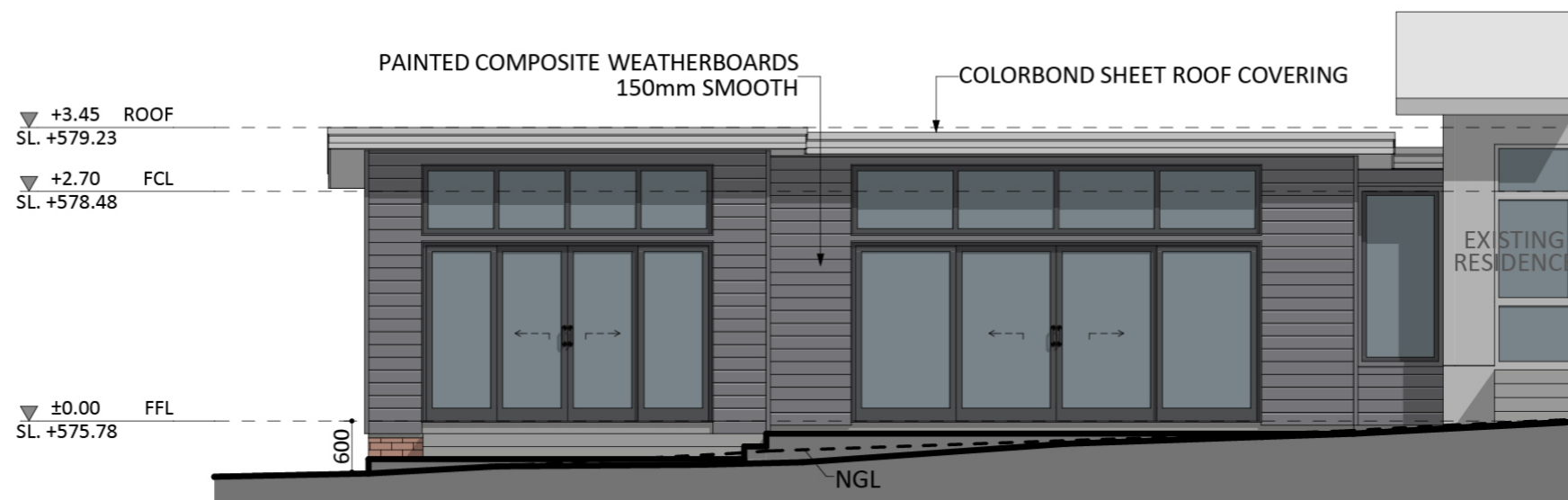
NORTH ELEVATION
