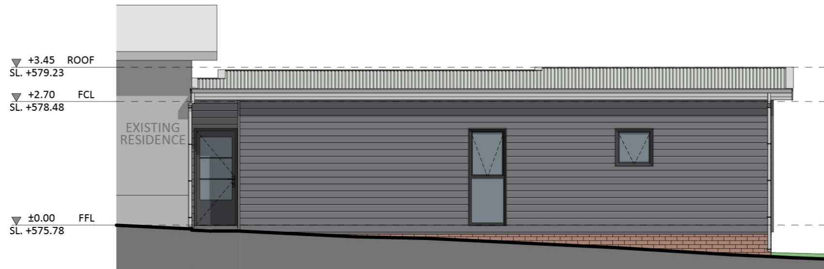
SOUTH ELEVATION
