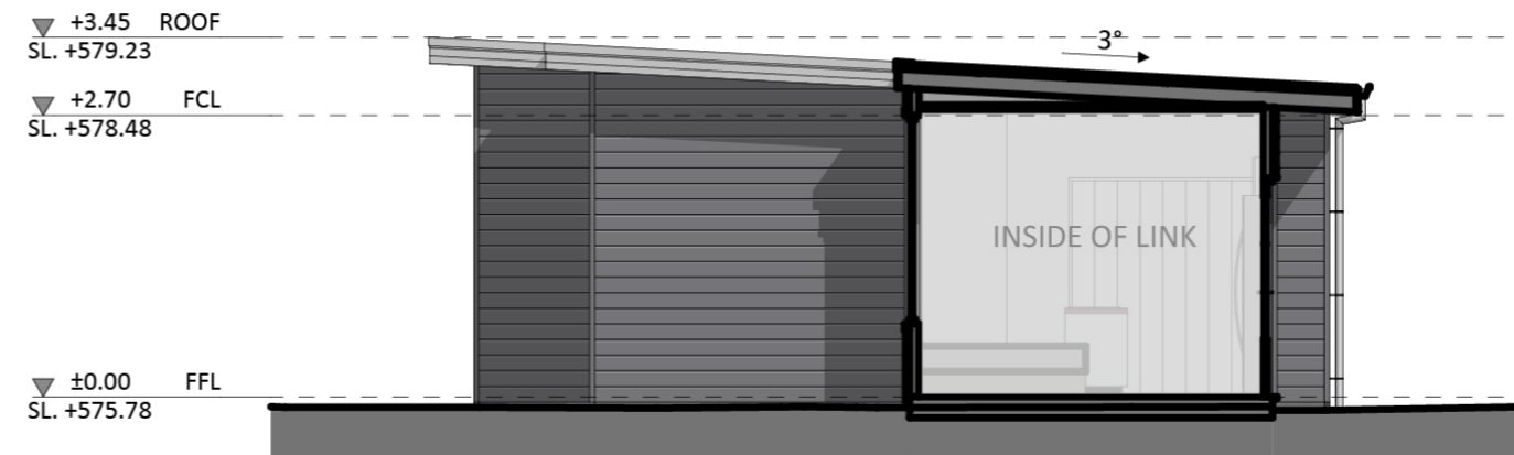
WEST ELEVATION
