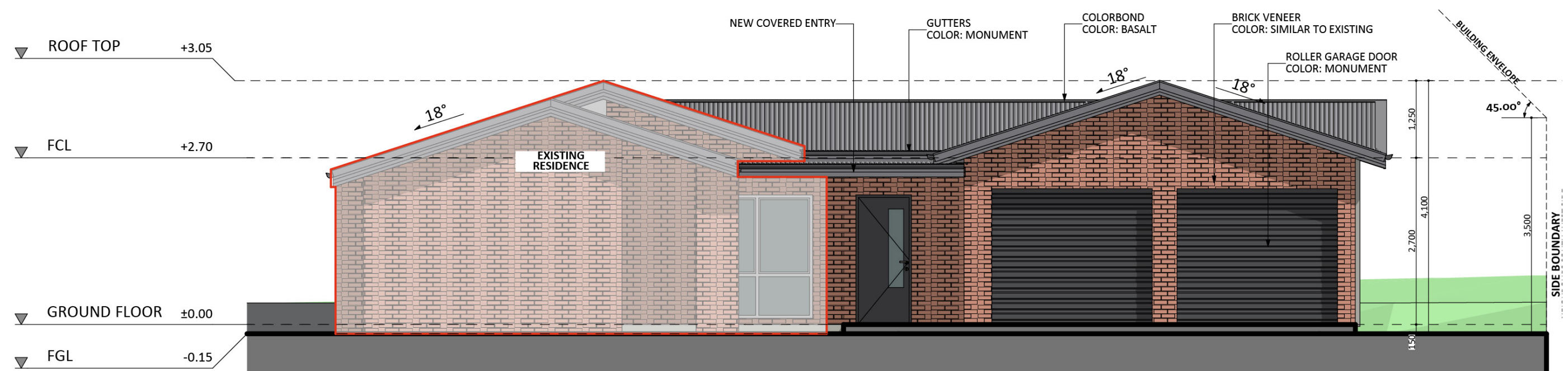
SOUTH-EAST ELEVATION
