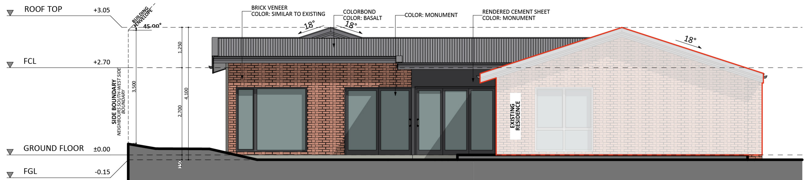
NORTH-WEST ELEVATION
