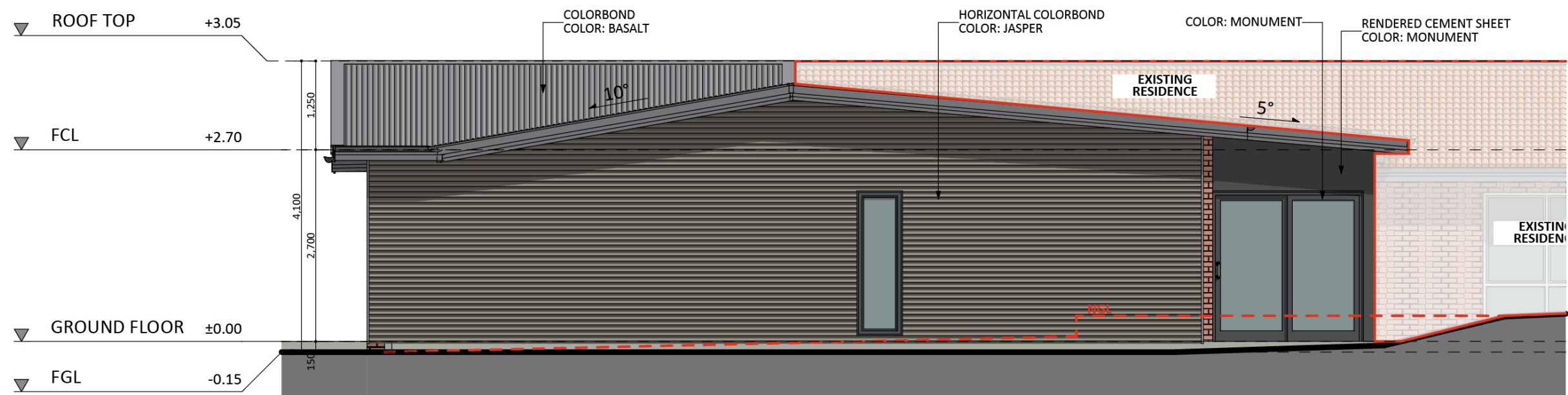
NORTH-EAST ELEVATION
