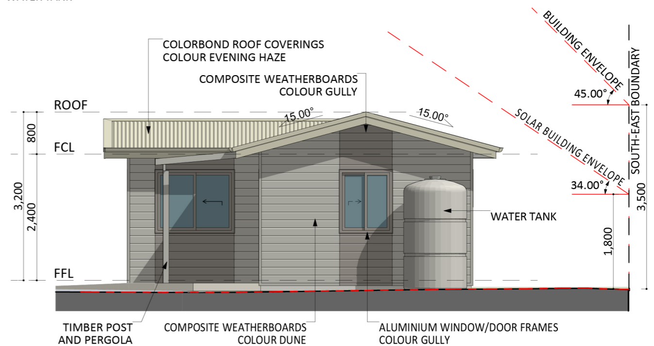
WEST ELEVATION
