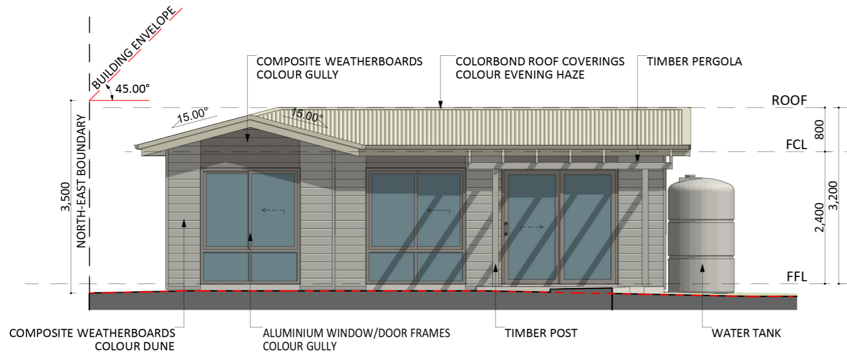
NORTH ELEVATION
