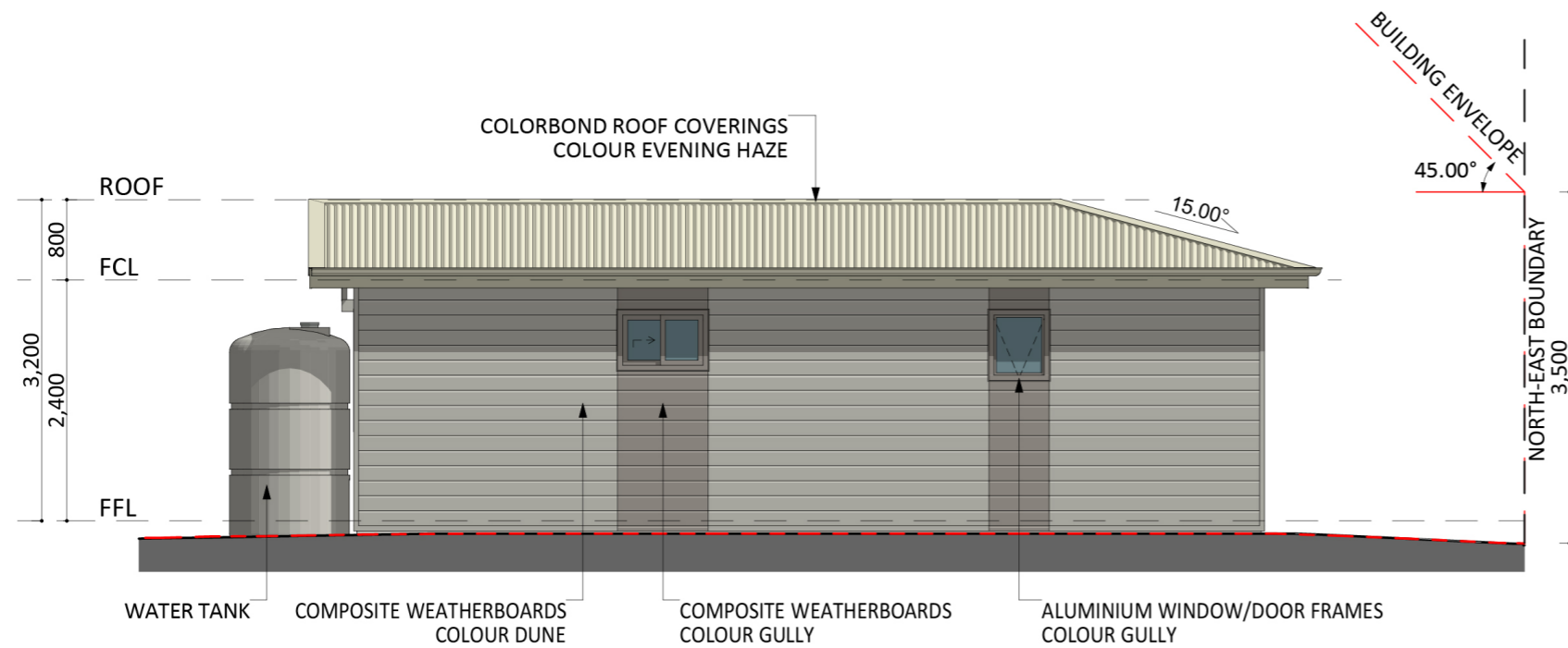
SOUTH ELEVATION
