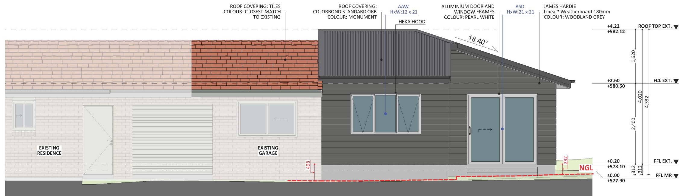
NORTH ELEV.
