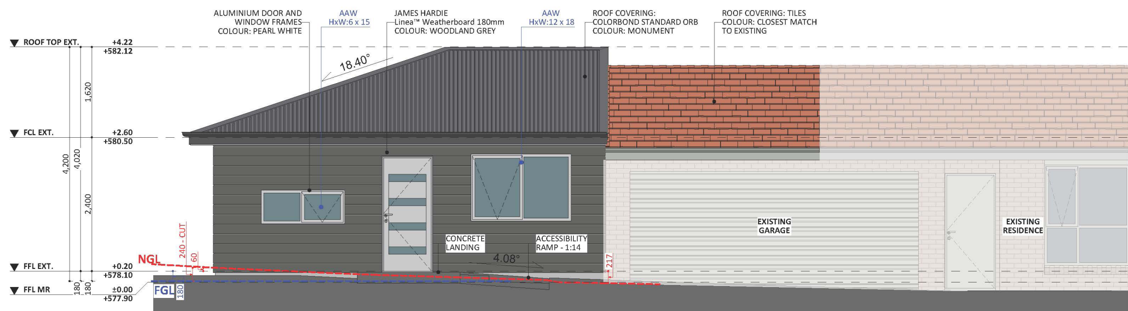
SOUTH ELEV.
