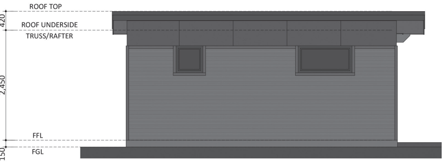
ELEVATION 03
