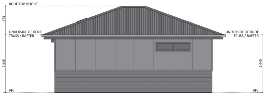
ELEVATION 03
